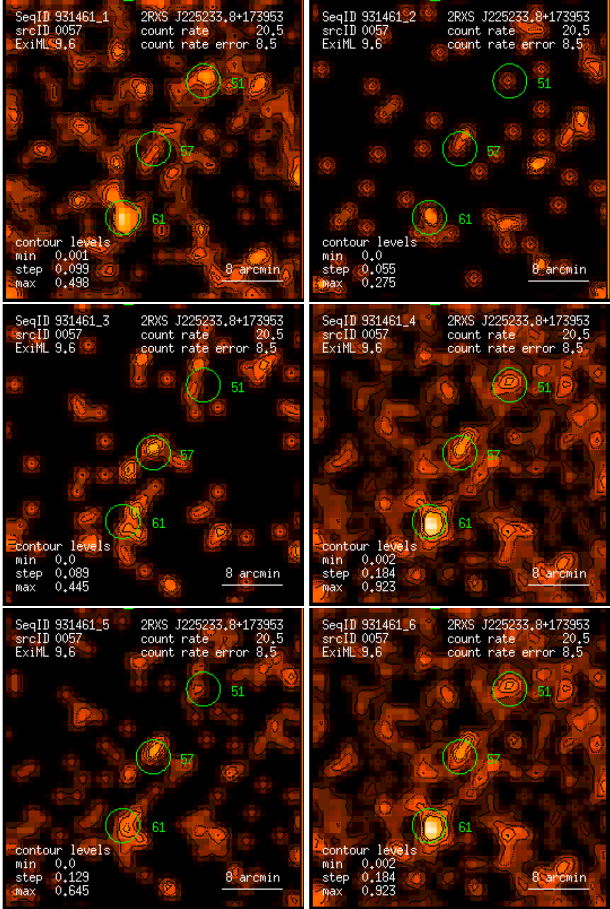
Figure 57: RASS 931461: detection 0057: band rate images, Gaussian filter: (1) PSPC channels 11 – 41, (2) 52 – 90, (3) 91 – 201, (4) 11 – 235, (5) 52 – 201, (6) 11 – 201. Broad band rates in counts/ks. Band rate contour levels in counts/ks/arcmin 2 .
