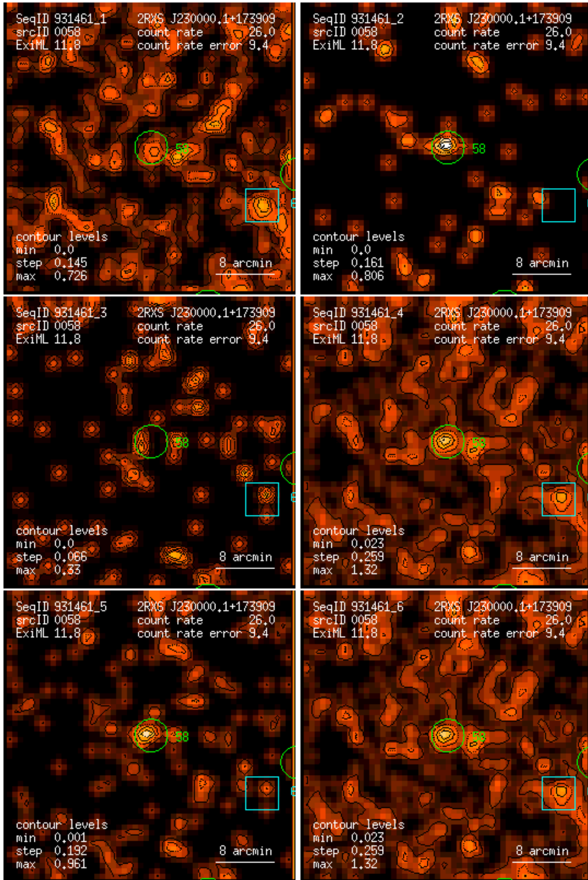
Figure 58: RASS 931461: detection 0058: band rate images, Gaussian filter: (1) PSPC channels 11 – 41, (2) 52 – 90, (3) 91 – 201, (4) 11 – 235, (5) 52 – 201, (6) 11 – 201. Broad band rates in counts/ks. Band rate contour levels in counts/ks/arcmin 2 .
