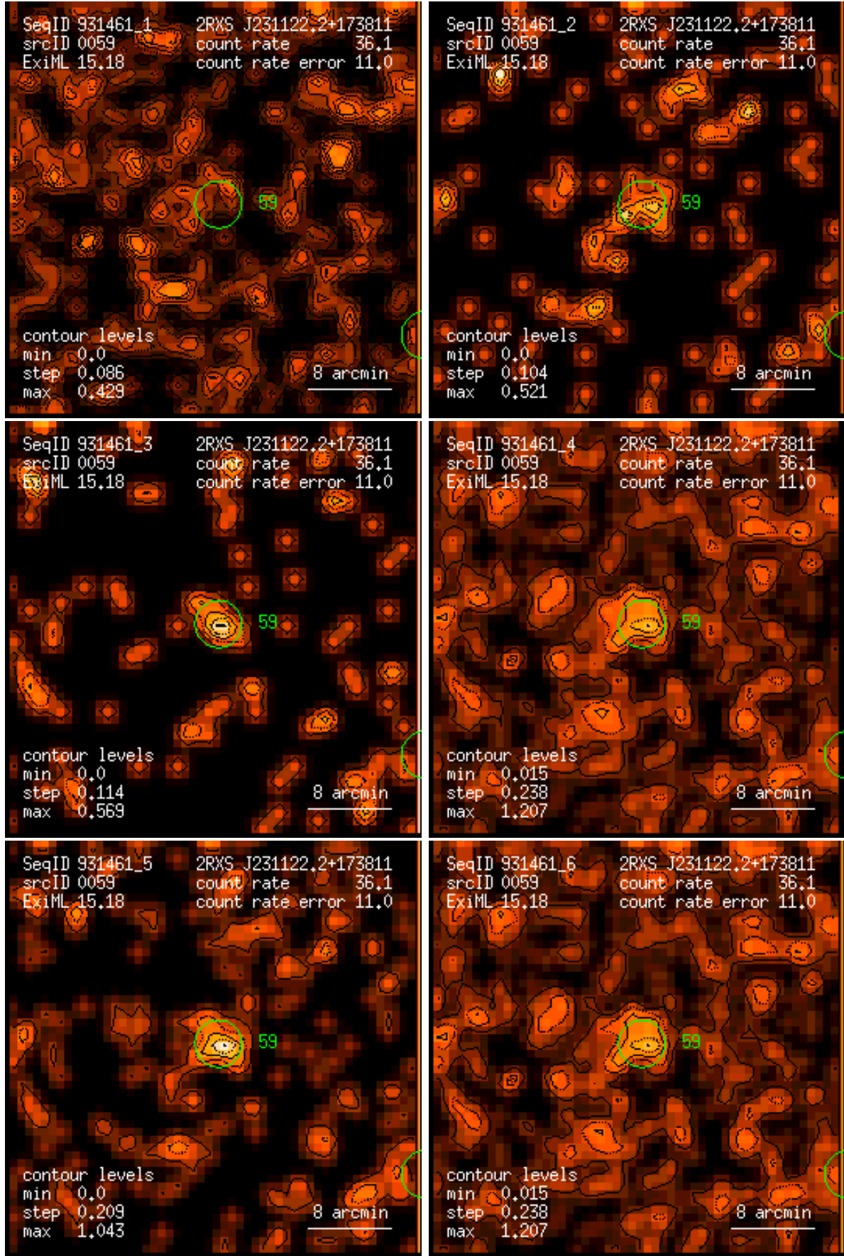
Figure 59: RASS 931461: detection 0059: band rate images, Gaussian filter: (1) PSPC channels 11 – 41, (2) 52 – 90, (3) 91 – 201, (4) 11 – 235, (5) 52 – 201, (6) 11 – 201. Broad band rates in counts/ks. Band rate contour levels in counts/ks/arcmin 2 .
