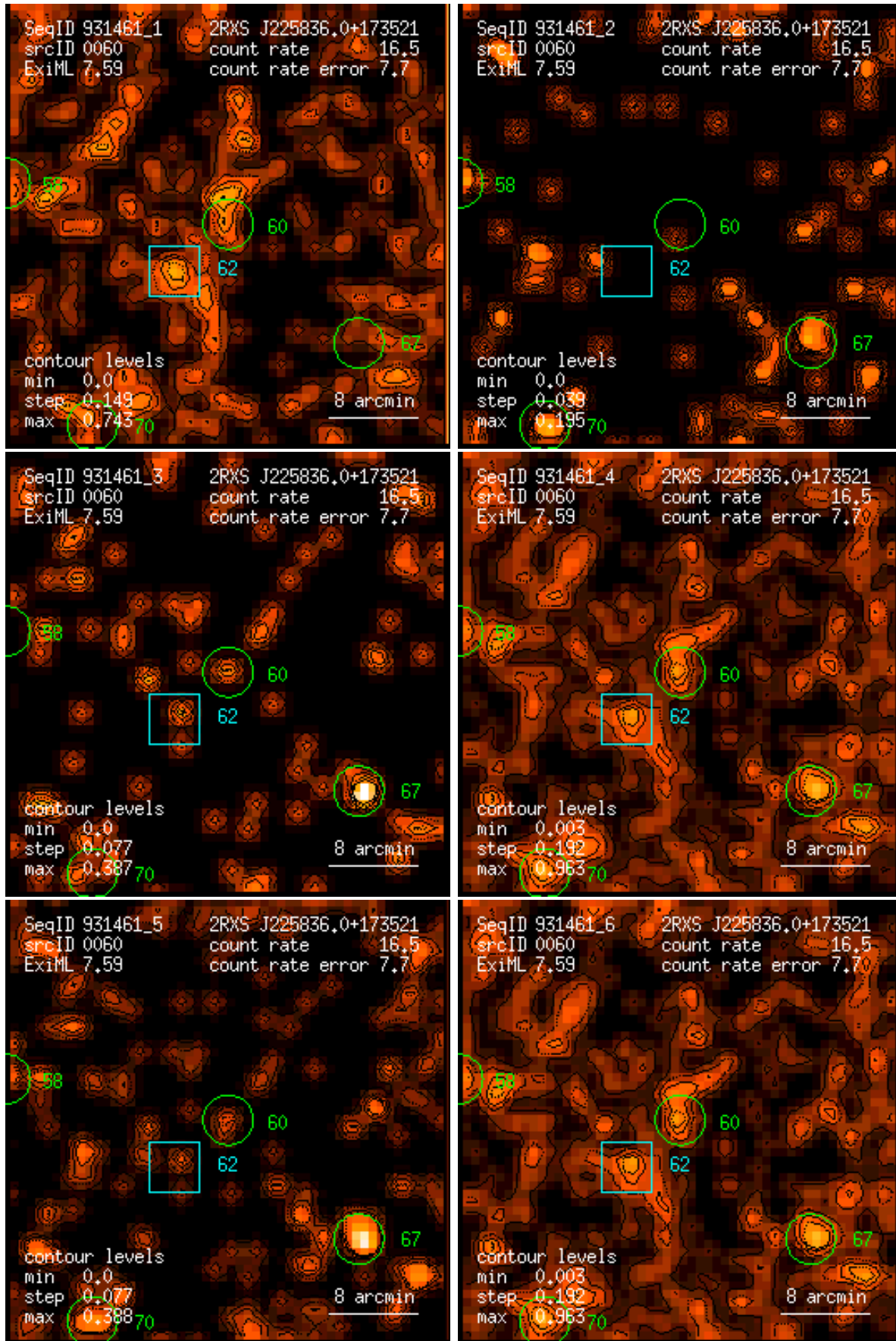
Figure 60: RASS 931461: detection 0060: band rate images, Gaussian filter: (1) PSPC channels 11 – 41, (2) 52 – 90, (3) 91 – 201, (4) 11 – 235, (5) 52 – 201, (6) 11 – 201. Broad band rates in counts/ks. Band rate contour levels in counts/ks/arcmin 2 .
