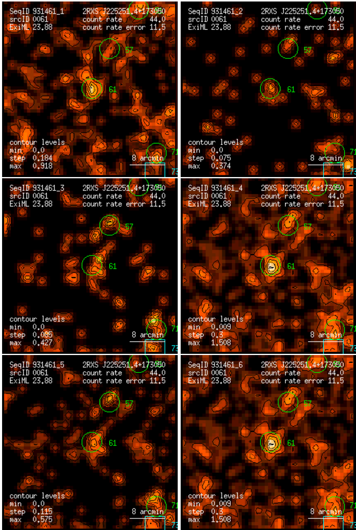
Figure 61: RASS 931461: detection 0061: band rate images, Gaussian filter: (1) PSPPC channels 11 – 41, (2) 52 – 90, (3) 91 – 201, (4) 11 – 235, (5) 52 – 201, (6) 11 – 201. Broad band rates in counts/ks. Band rate contour levels in counts/ks/arcmin 2 .
