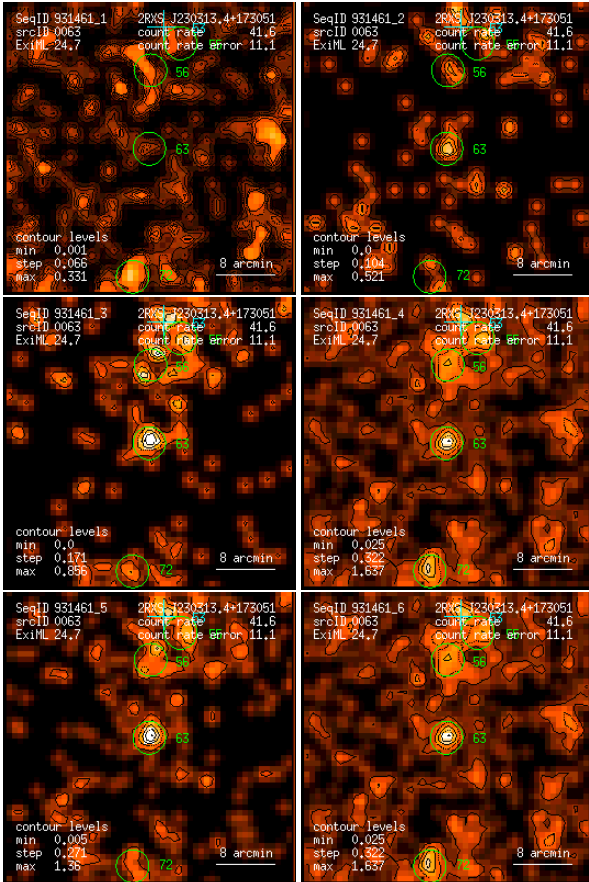
Figure 63: RASS 931461: detection 0063: band rate images, Gaussian filter: (1) PSPC channels 11 – 41, (2) 52 – 90, (3) 91 – 201, (4) 11 – 235, (5) 52 – 201, (6) 11 – 201. Broad band rates in counts/ks. Band rate contour levels in counts/ks/arcmin 2 .
