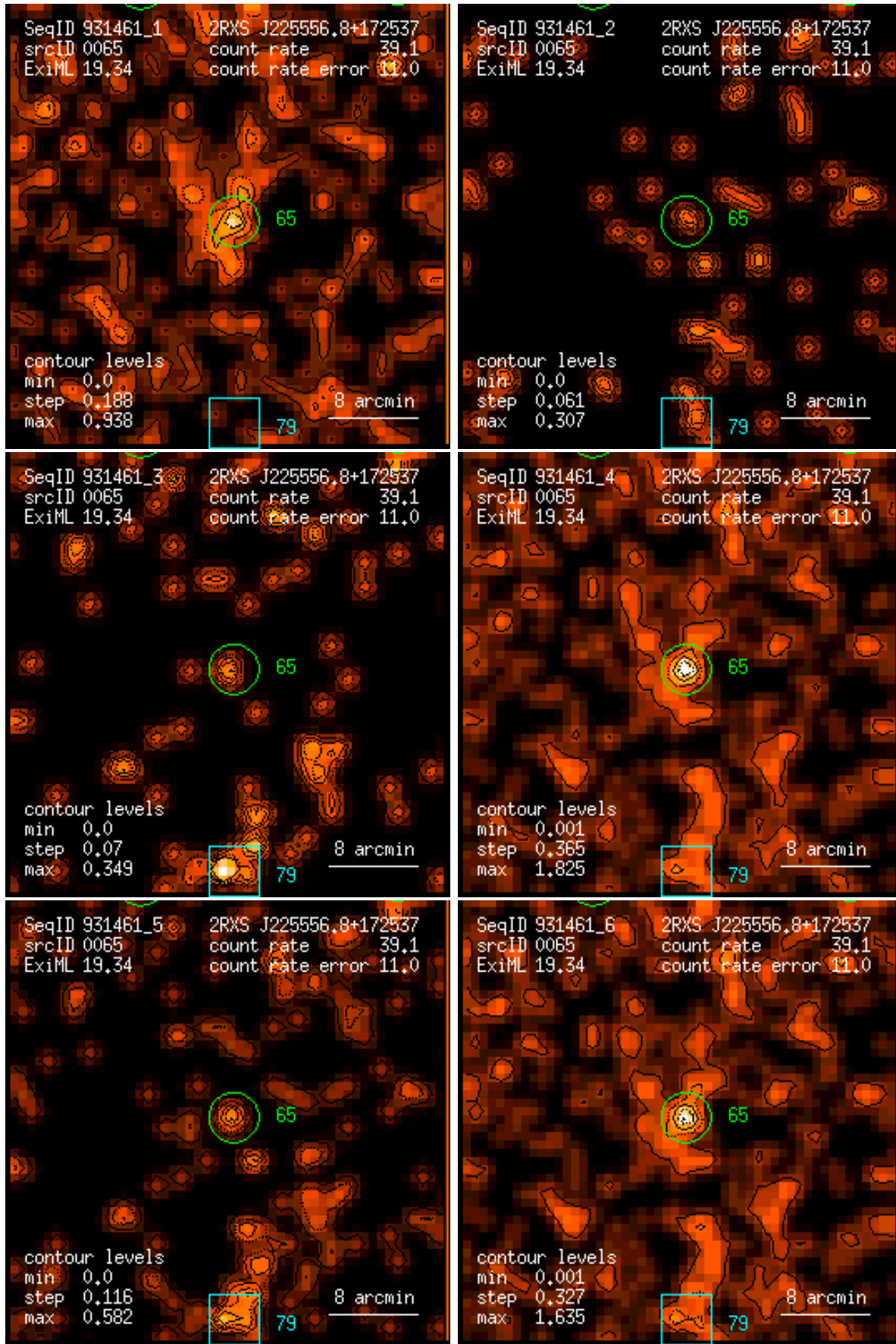
Figure 65: RASS 931461: detection 0065: band rate images, Gaussian filter: (1) PSPC channels 11 – 41, (2) 52 – 90, (3) 91 – 201, (4) 11 – 235, (5) 52 – 201, (6) 11 – 201. Broad band rates in counts/ks. Band rate contour levels in counts/ks/arcmin 2 .
