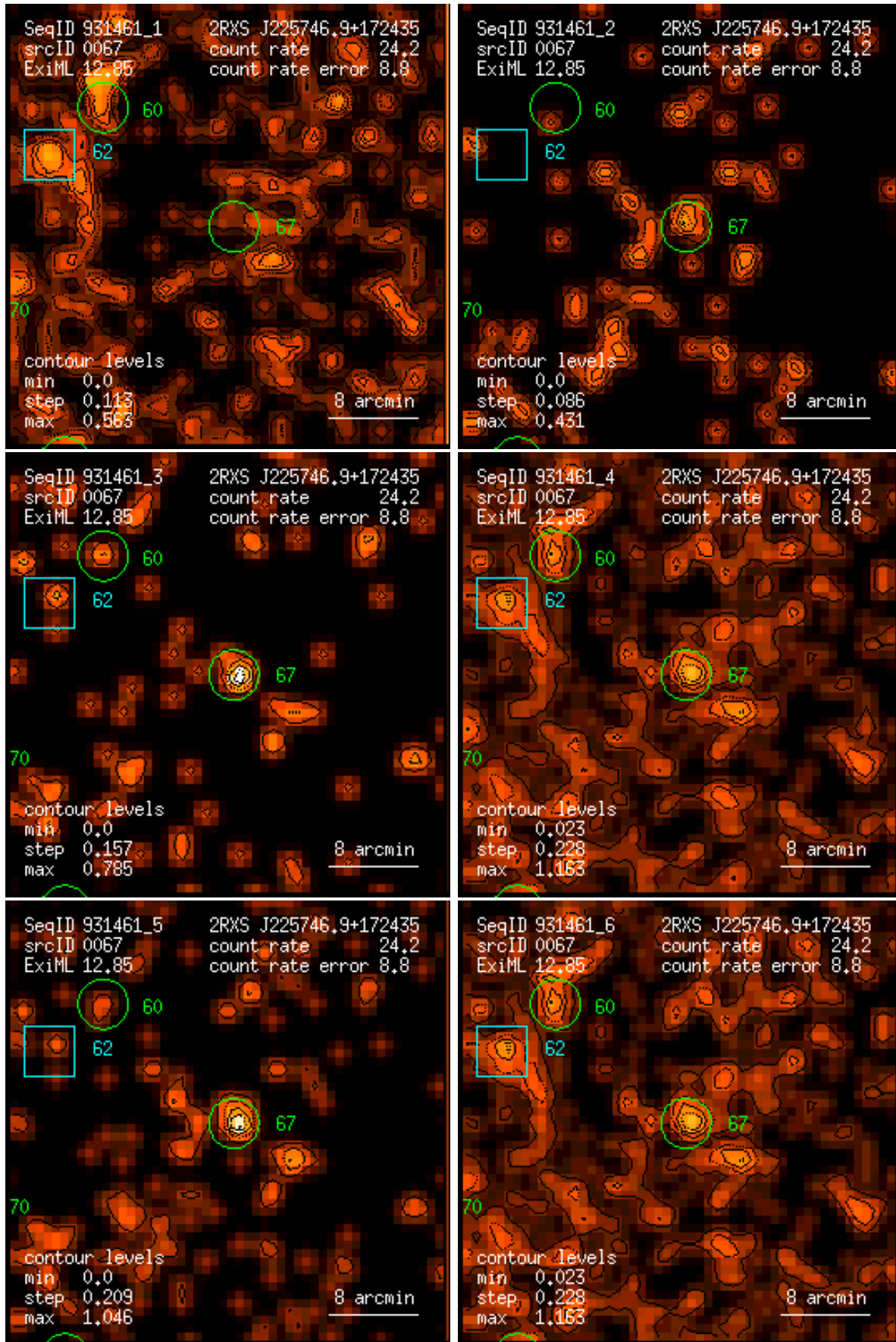
Figure 67: RASS 931461: detection 0067: band rate images, Gaussian filter: (1) PSPC channels 11 – 41, (2) 52 – 90, (3) 91 – 201, (4) 11 – 235, (5) 52 – 201, (6) 11 – 201. Broad band rates in counts/ks. Band rate contour levels in counts/ks/arcmin 2 .
