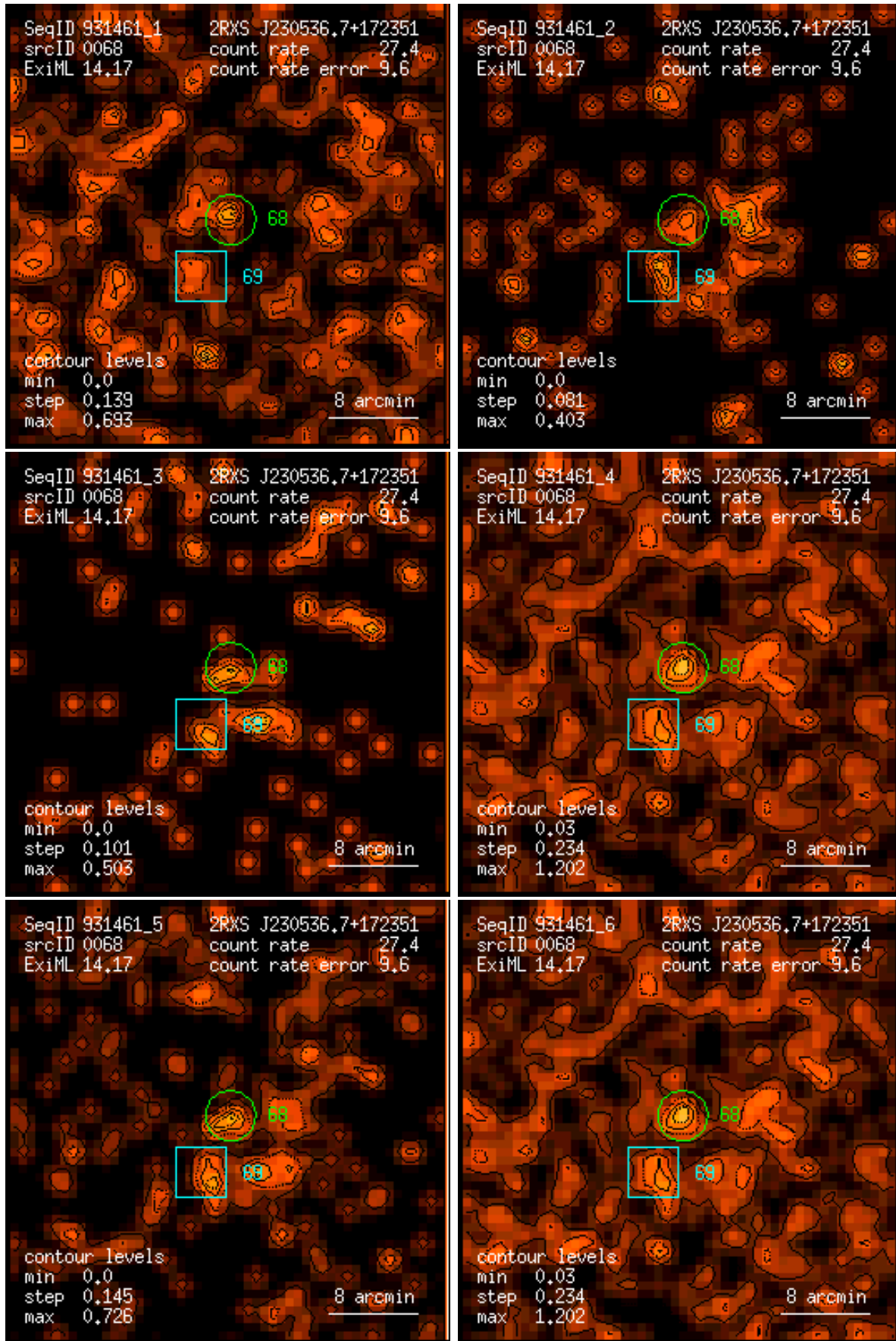
Figure 68: RASS 931461: detection 0068: band rate images, Gaussian filter: (1) PSPC channels 11 – 41, (2) 52 – 90, (3) 91 – 201, (4) 11 – 235, (5) 52 – 201, (6) 11 – 201. Broad band rates in counts/ks. Band rate contour levels in counts/ks/arcmin 2 .
