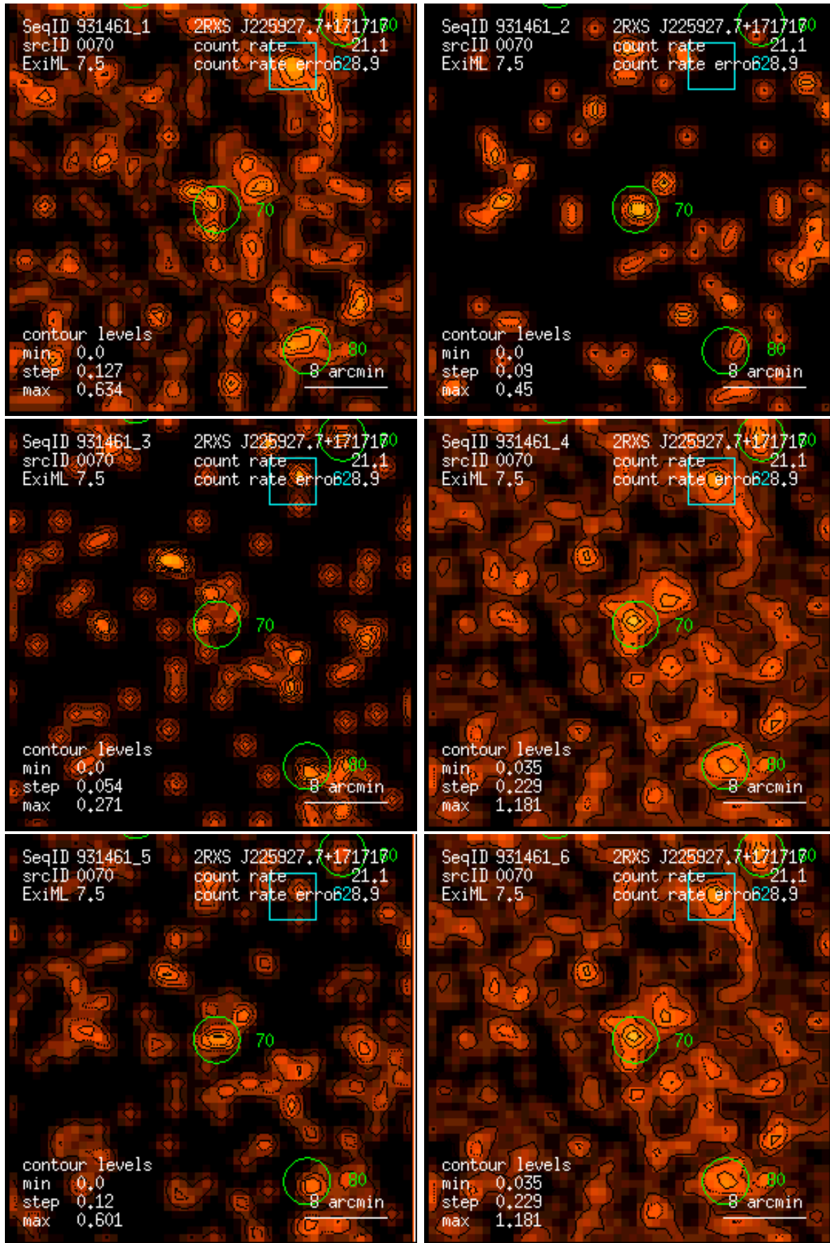
Figure 70: RASS 931461: detection 0070: band rate images, Gaussian filter: (1) PSPC channels 11 – 41, (2) 52 – 90, (3) 91 – 201, (4) 11 – 235, (5) 52 – 201, (6) 11 – 201. Broad band rates in counts/ks. Band rate contour levels in counts/ks/arcmin 2 .
