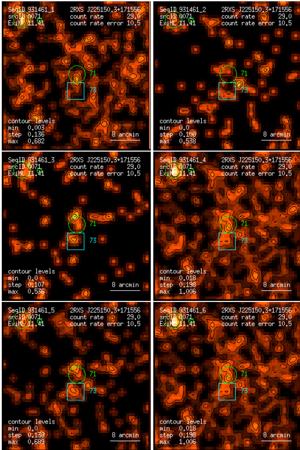
Figure 71: RASS 931461: detection 0071: band rate images, Gaussian filter: (1) PSPC channels 11 – 41, (2) 52 – 90, (3) 91 – 201, (4) 11 – 235, (5) 52 – 201, (6) 11 – 201. Broad band rates in counts/ks. Band rate contour levels in counts/ks/arcmin 2 .
