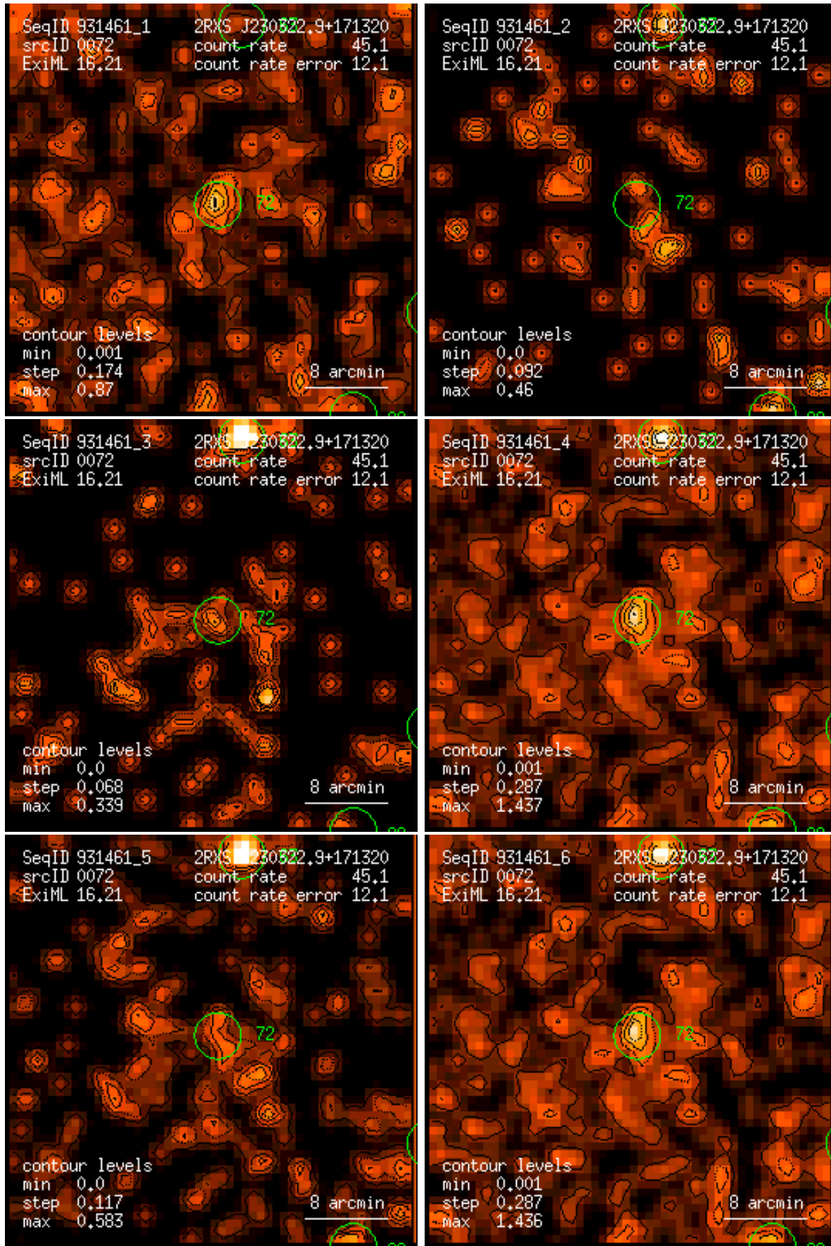
Figure 72: RASS 931461: detection 0072: band rate images, Gaussian filter: (1) PSPC channels 11 – 41, (2) 52 – 90, (3) 91 – 201, (4) 11 – 235, (5) 52 – 201, (6) 11 – 201. Broad band rates in counts/ks. Band rate contour levels in counts/ks/arcmin 2 .
