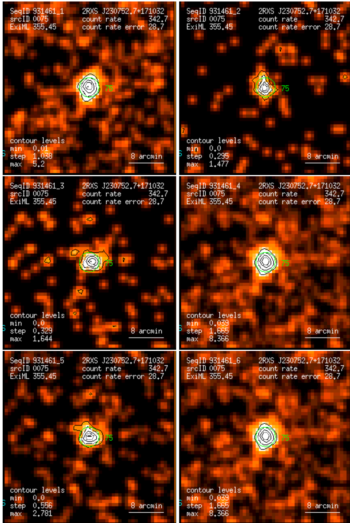
Figure 75: RASS 931461: detection 0075: band rate images, Gaussian filter: (1) PSPC channels 11 – 41, (2) 52 – 90, (3) 91 – 201, (4) 11 – 235, (5) 52 – 201, (6) 11 – 201. Broad band rates in counts/ks. Band rate contour levels in counts/ks/arcmin 2 .
