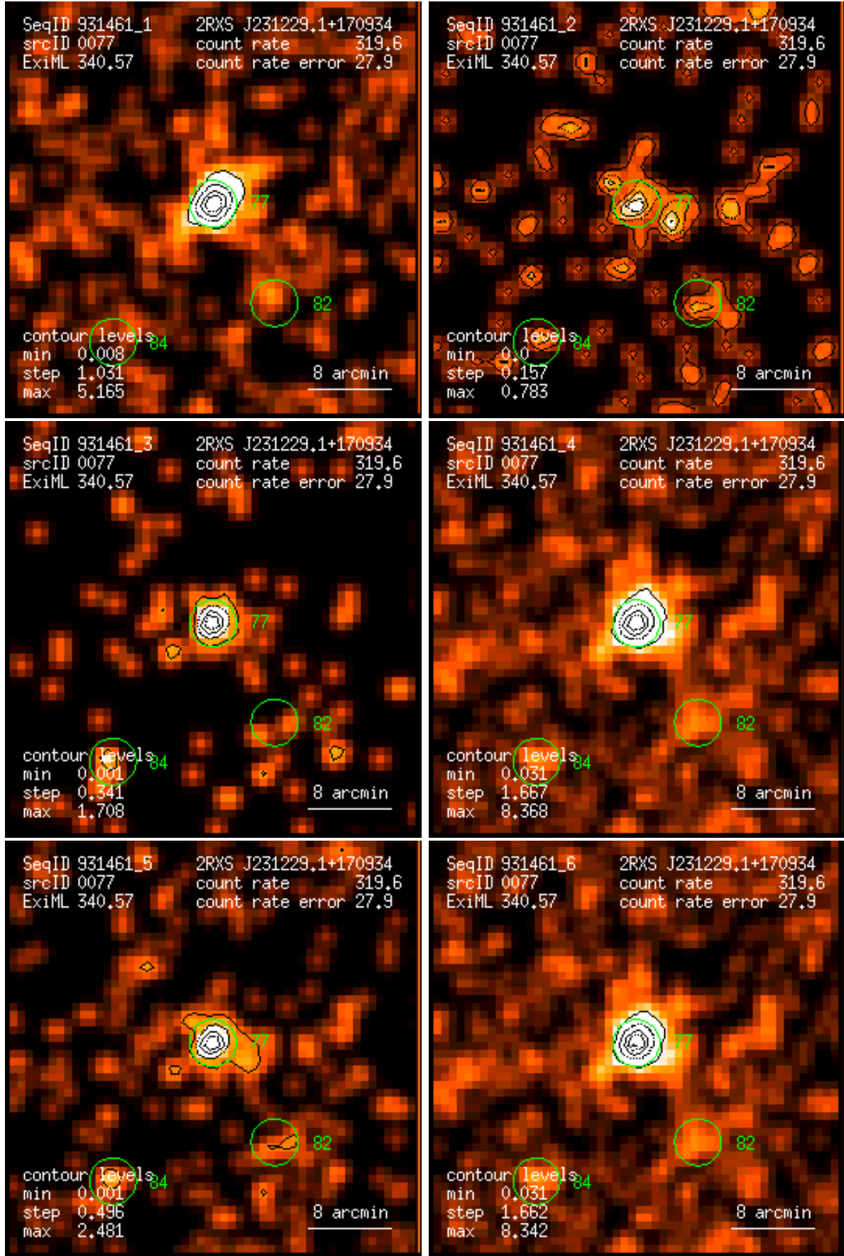
Figure 77: RASS 931461: detection 0077: band rate images, Gaussian filter: (1) PSPC channels 11 – 41, (2) 52 – 90, (3) 91 – 201, (4) 11 – 235, (5) 52 – 201, (6) 11 – 201. Broad band rates in counts/ks. Band rate contour levels in counts/ks/arcmin 2 .
