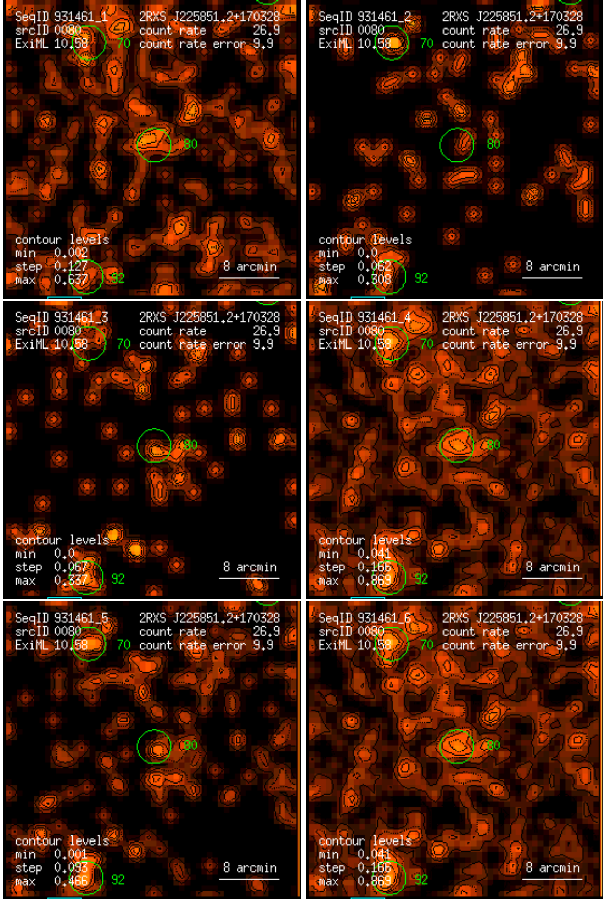
Figure 80: RASS 931461: detection 0080: band rate images, Gaussian filter: (1) PSPC channels 11 – 41, (2) 52 – 90, (3) 91 – 201, (4) 11 – 235, (5) 52 – 201, (6) 11 – 201. Broad band rates in counts/ks. Band rate contour levels in counts/ks/arcmin 2 .
