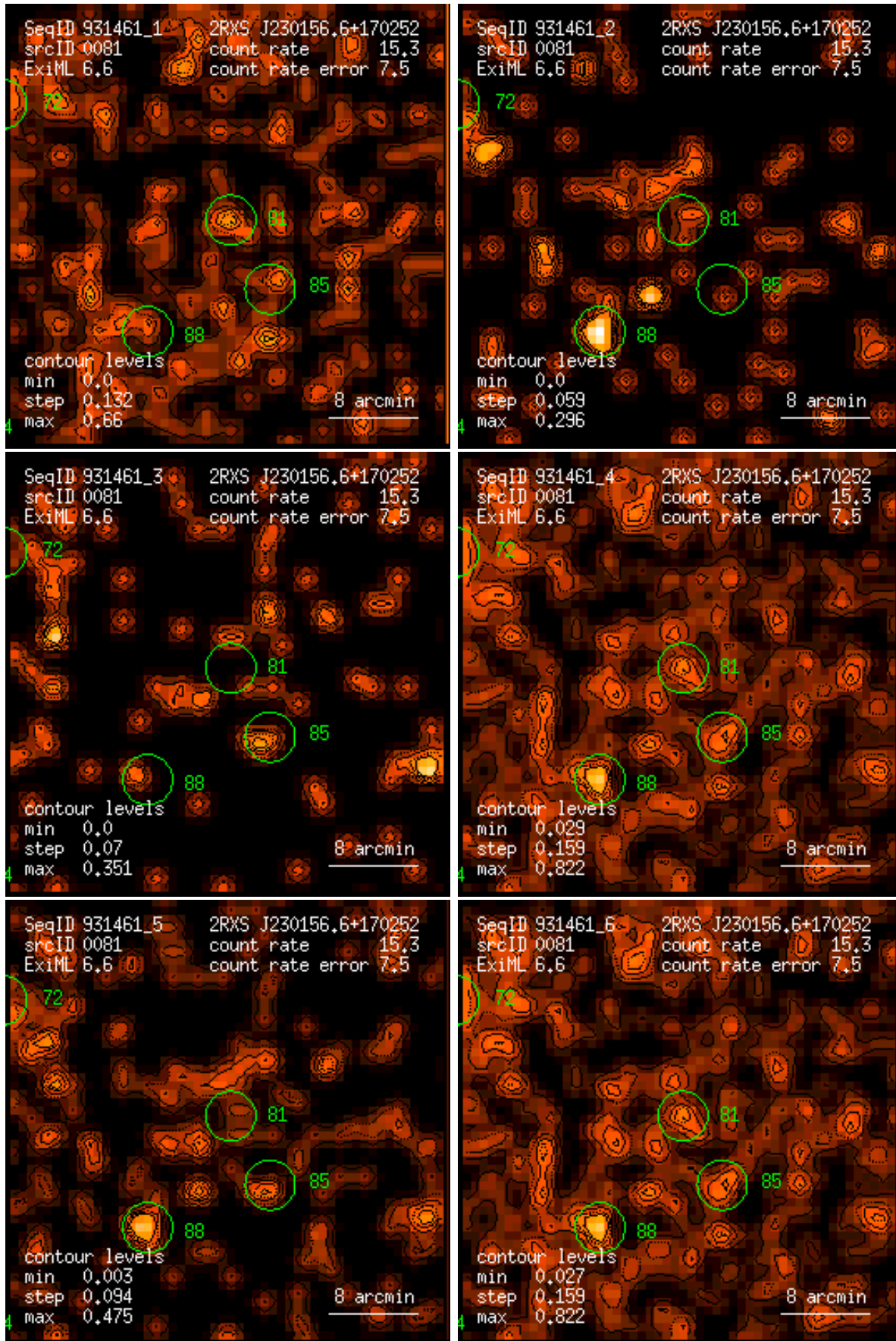
Figure 81: RASS 931461: detection 0081: band rate images, Gaussian filter: (1) PSPC channels 11 – 41, (2) 52 – 90, (3) 91 – 201, (4) 11 – 235, (5) 52 – 201, (6) 11 – 201. Broad band rates in counts/ks. Band rate contour levels in counts/ks/arcmin 2 .
