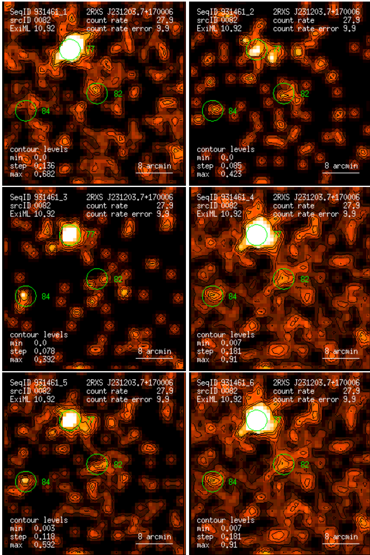
Figure 82: RASS 931461: detection 0082: band rate images, Gaussian filter: (1) PSPC channels 11 – 41, (2) 52 – 90, (3) 91 – 201, (4) 11 – 235, (5) 52 – 201, (6) 11 – 201. Broad band rates in counts/ks. Band rate contour levels in counts/ks/arcmin 2 .
