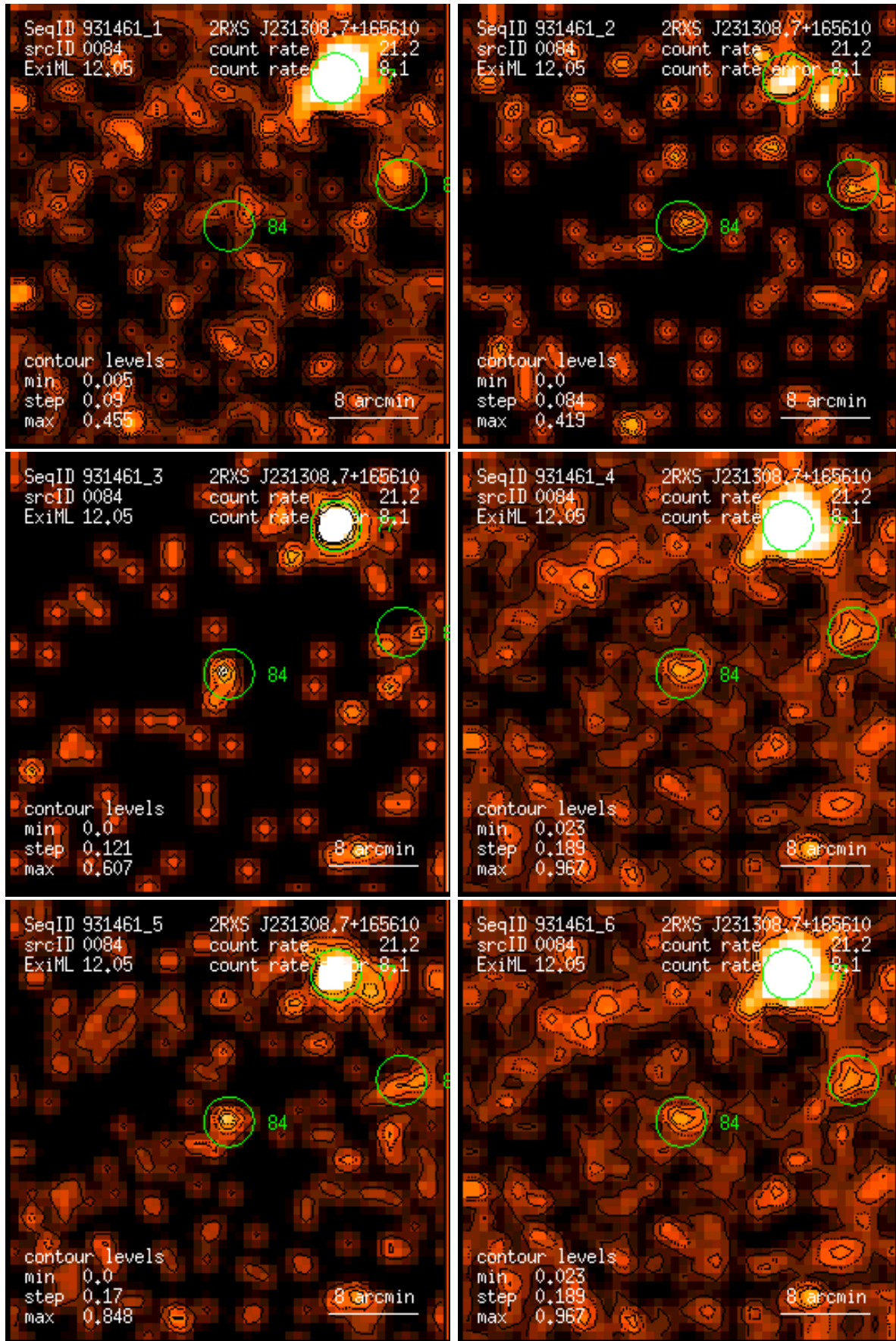
Figure 84: RASS 931461: detection 0084: band rate images, Gaussian filter: (1) PSPC channels 11 – 41, (2) 52 – 90, (3) 91 – 201, (4) 11 – 235, (5) 52 – 201, (6) 11 – 201. Broad band rates in counts/ks. Band rate contour levels in counts/ks/arcmin 2 .
