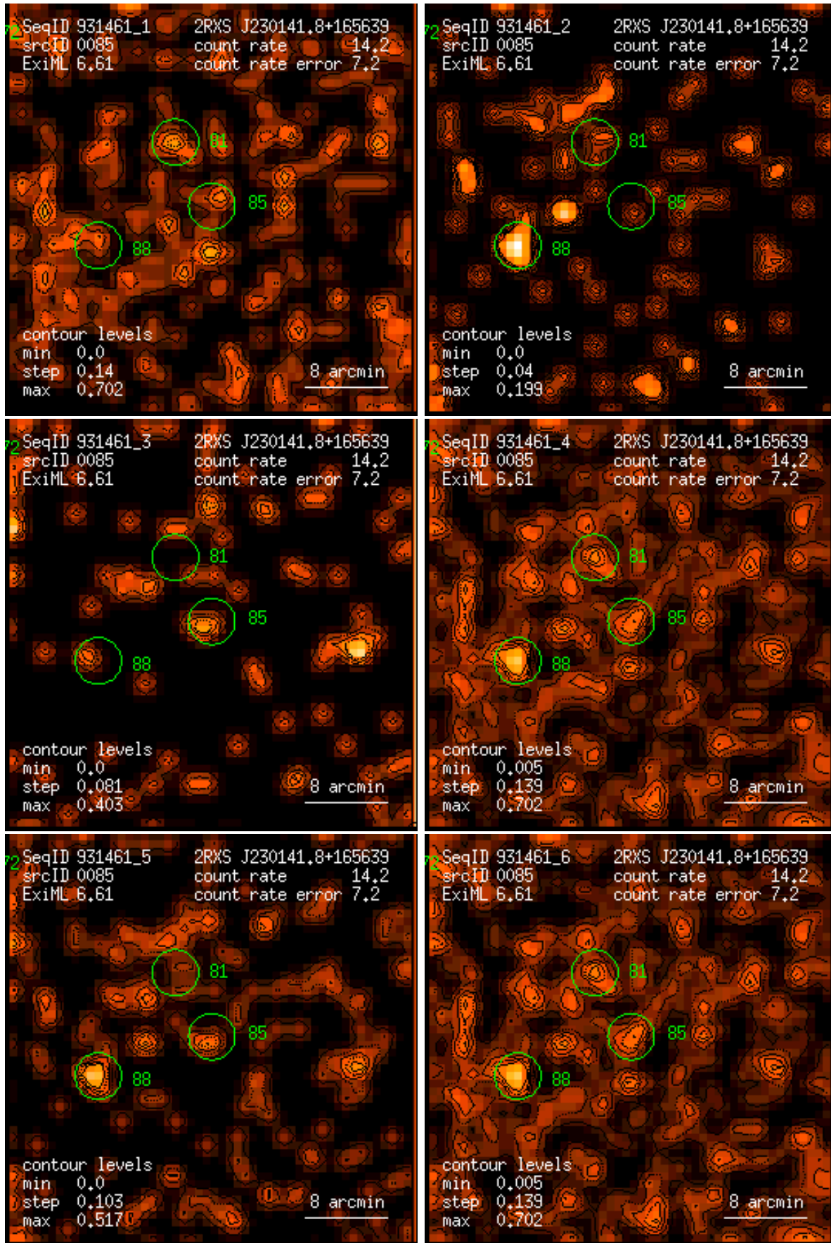
Figure 85: RASS 931461: detection 0085: band rate images, Gaussian filter: (1) PSPC channels 11 – 41, (2) 52 – 90, (3) 91 – 201, (4) 11 – 235, (5) 52 – 201, (6) 11 – 201. Broad band rates in counts/ks. Band rate contour levels in counts/ks/arcmin 2 .
