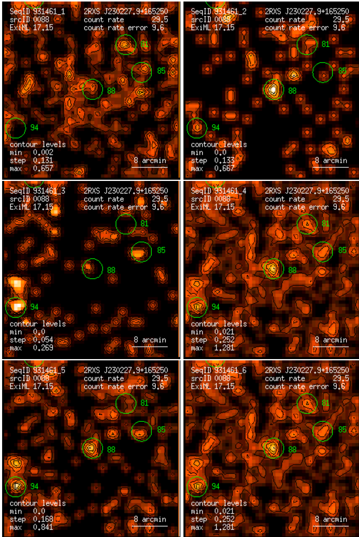
Figure 88: RASS 931461: detection 0088: band rate images, Gaussian filter: (1) PSPC channels 11 – 41, (2) 52 – 90, (3) 91 – 201, (4) 11 – 235, (5) 52 – 201, (6) 11 – 201. Broad band rates in counts/ks. Band rate contour levels in counts/ks/arcmin 2 .
