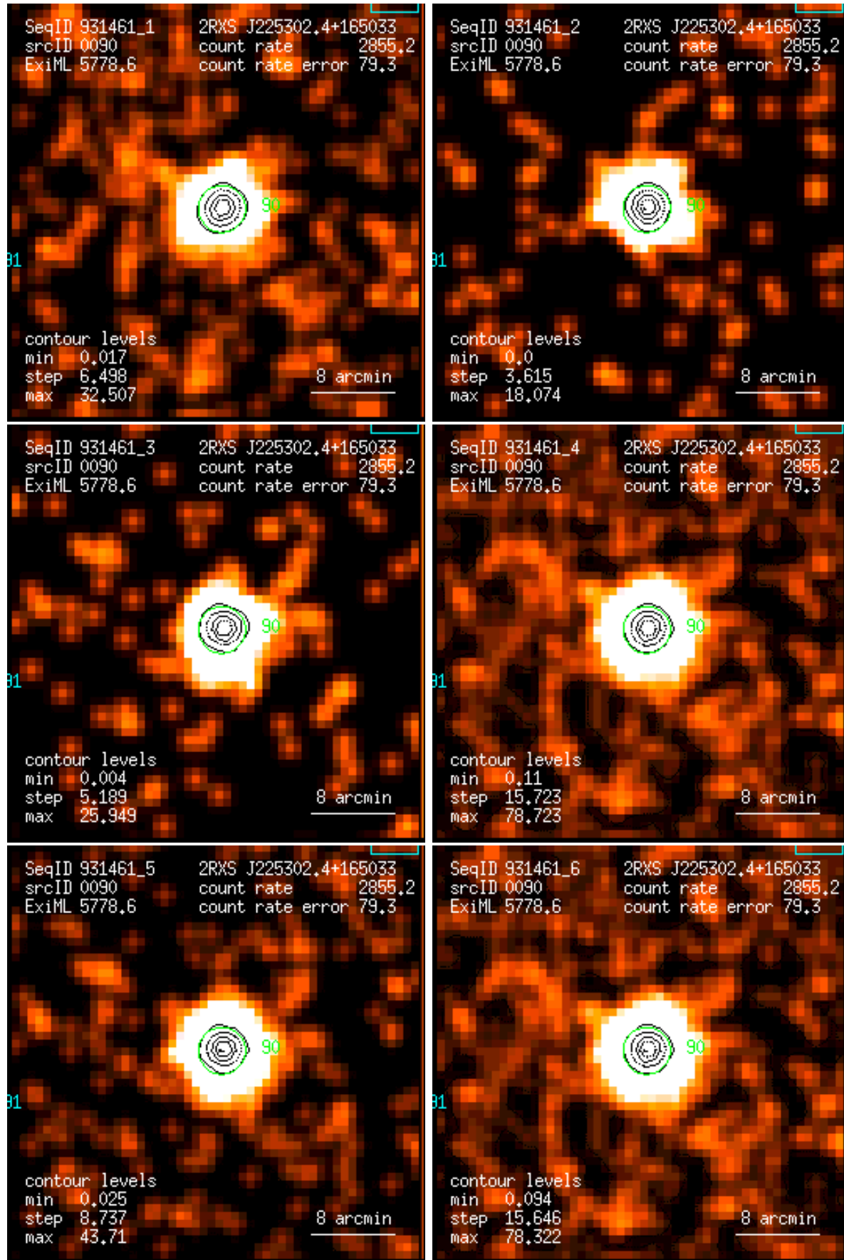
Figure 90: RASS 931461: detection 0090: band rate images, Gaussian filter: (1) PSPC channels 11 – 41, (2) 52 – 90, (3) 91 – 201, (4) 11 – 235, (5) 52 – 201, (6) 11 – 201. Broad band rates in counts/ks. Band rate contour levels in counts/ks/arcmin 2 .
