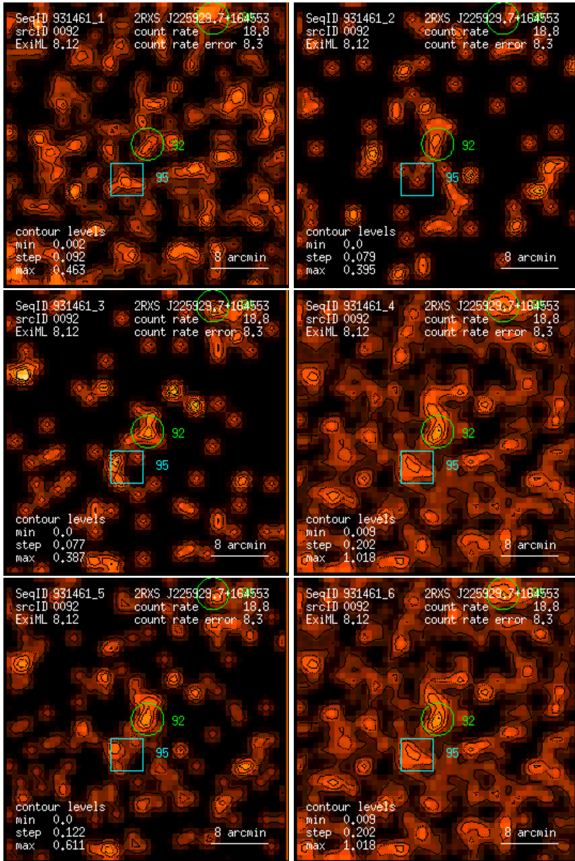
Figure 92: RASS 931461: detection 0092: band rate images, Gaussian filter: (1) PSPC channels 11 – 41, (2) 52 – 90, (3) 91 – 201, (4) 11 – 235, (5) 52 – 201, (6) 11 – 201. Broad band rates in counts/ks. Band rate contour levels in counts/ks/arcmin 2 .
