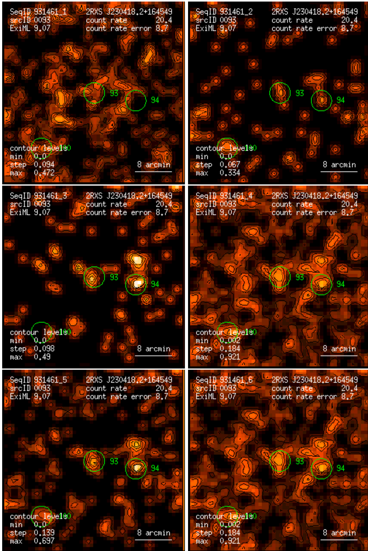
Figure 93: RASS 931461: detection 0093: band rate images, Gaussian filter: (1) PSPC channels 11 – 41, (2) 52 – 90, (3) 91 – 201, (4) 11 – 235, (5) 52 – 201, (6) 11 – 201. Broad band rates in counts/ks. Band rate contour levels in counts/ks/arcmin 2 .
