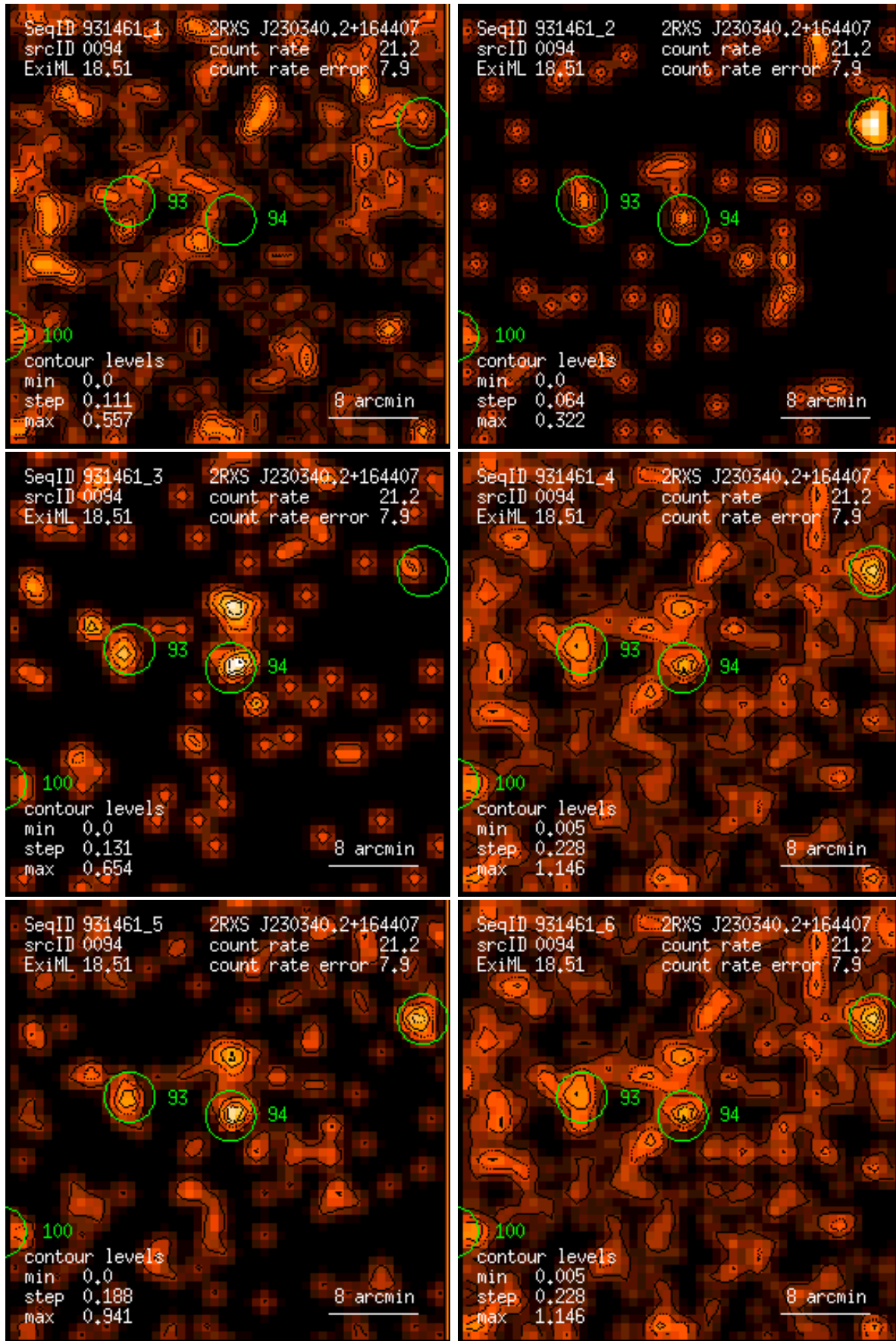
Figure 94: RASS 931461: detection 0094: band rate images, Gaussian filter: (1) PSPC channels 11 – 41, (2) 52 – 90, (3) 91 – 201, (4) 11 – 235, (5) 52 – 201, (6) 11 – 201. Broad band rates in counts/ks. Band rate contour levels in counts/ks/arcmin 2 .
