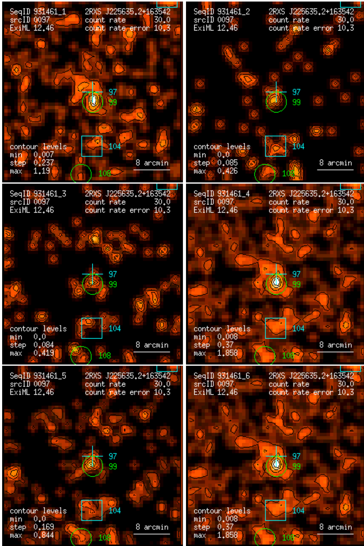
Figure 97: RASS 931461: detection 0097: band rate images, Gaussian filter: (1) PSPC channels 11 – 41, (2) 52 – 90, (3) 91 – 201, (4) 11 – 235, (5) 52 – 201, (6) 11 – 201. Broad band rates in counts/ks. Band rate contour levels in counts/ks/arcmin 2 .
