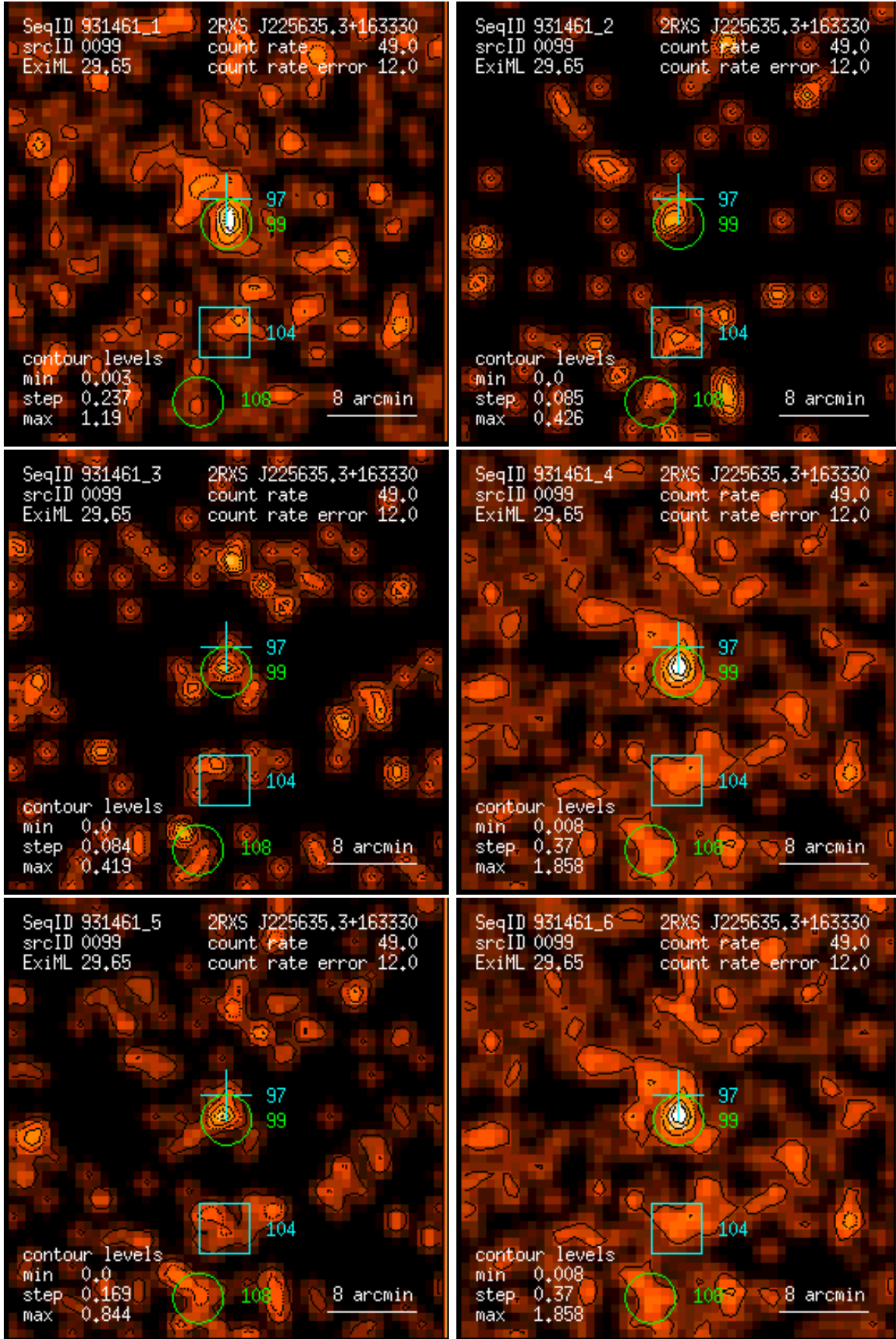
Figure 99: RASS 931461: detection 0099: band rate images, Gaussian filter: (1) PSC channels 11 – 41, (2) 52 – 90, (3) 91 – 201, (4) 11 – 235, (5) 52 – 201, (6) 11 – 201. Broad band rates in counts/ks. Band rate contour levels in counts/ks/arcmin 2 .
