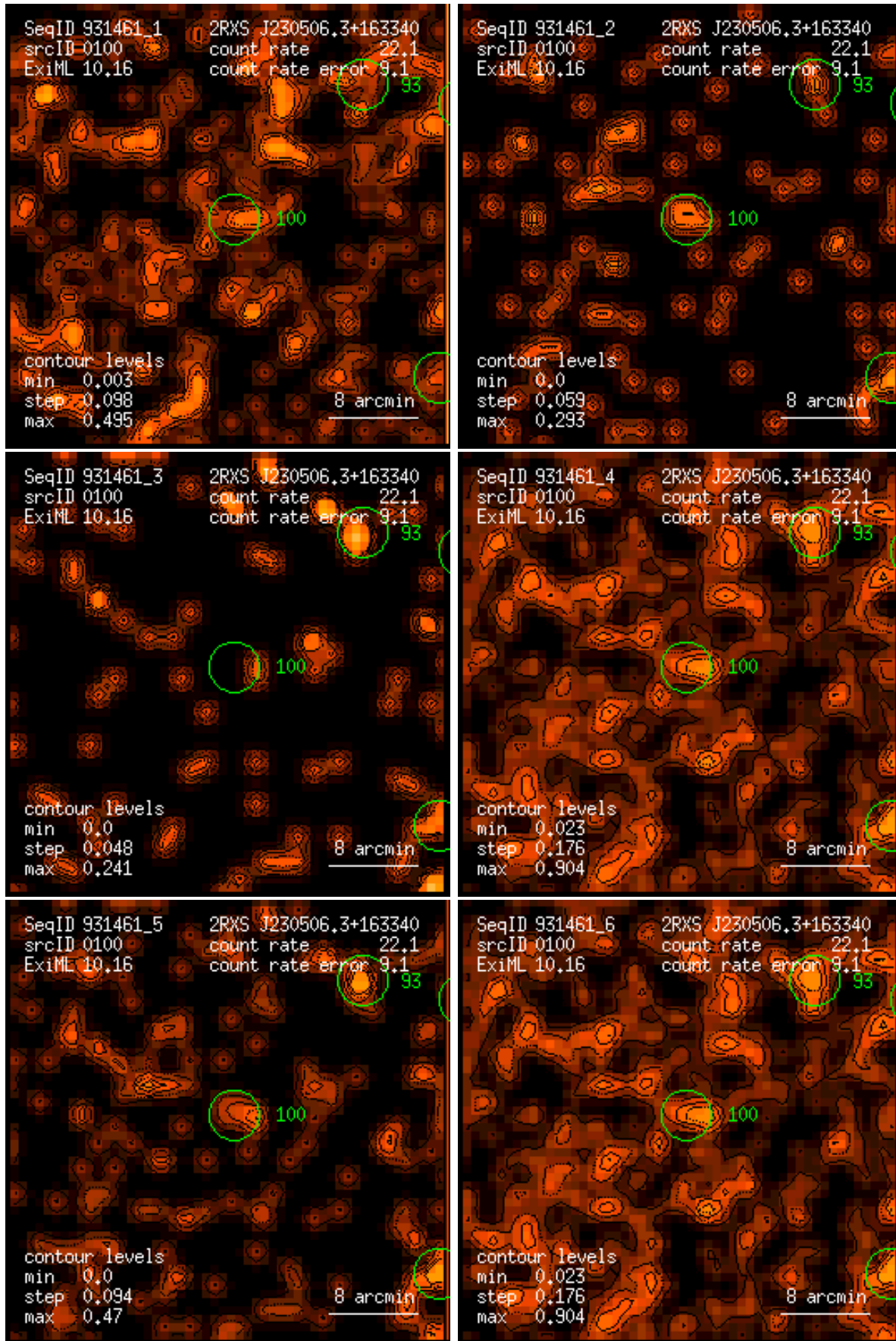
Figure 100: RASS 931461: detection 0100: band rate images, Gaussian filter: (1) PSPC channels 11 – 41, (2) 52 – 90, (3) 91 – 201, (4) 11 – 235, (5) 52 – 201, (6) 11 – 201. Broad band rates in counts/ks. Band rate contour levels in counts/ks/arcmin 2 .
