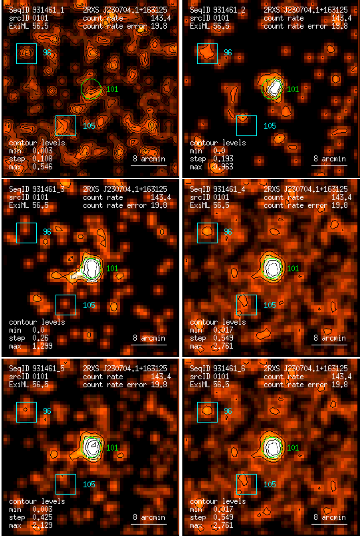
Figure 101: RASS 931461: detection 0101: band rate images, Gaussian filter: (1) PSPC channels 11 – 41, (2) 52 – 90, (3) 91 – 201, (4) 11 – 235, (5) 52 – 201, (6) 11 – 201. Broad band rates in counts/ks. Band rate contour levels in counts/ks/arcmin 2 .
