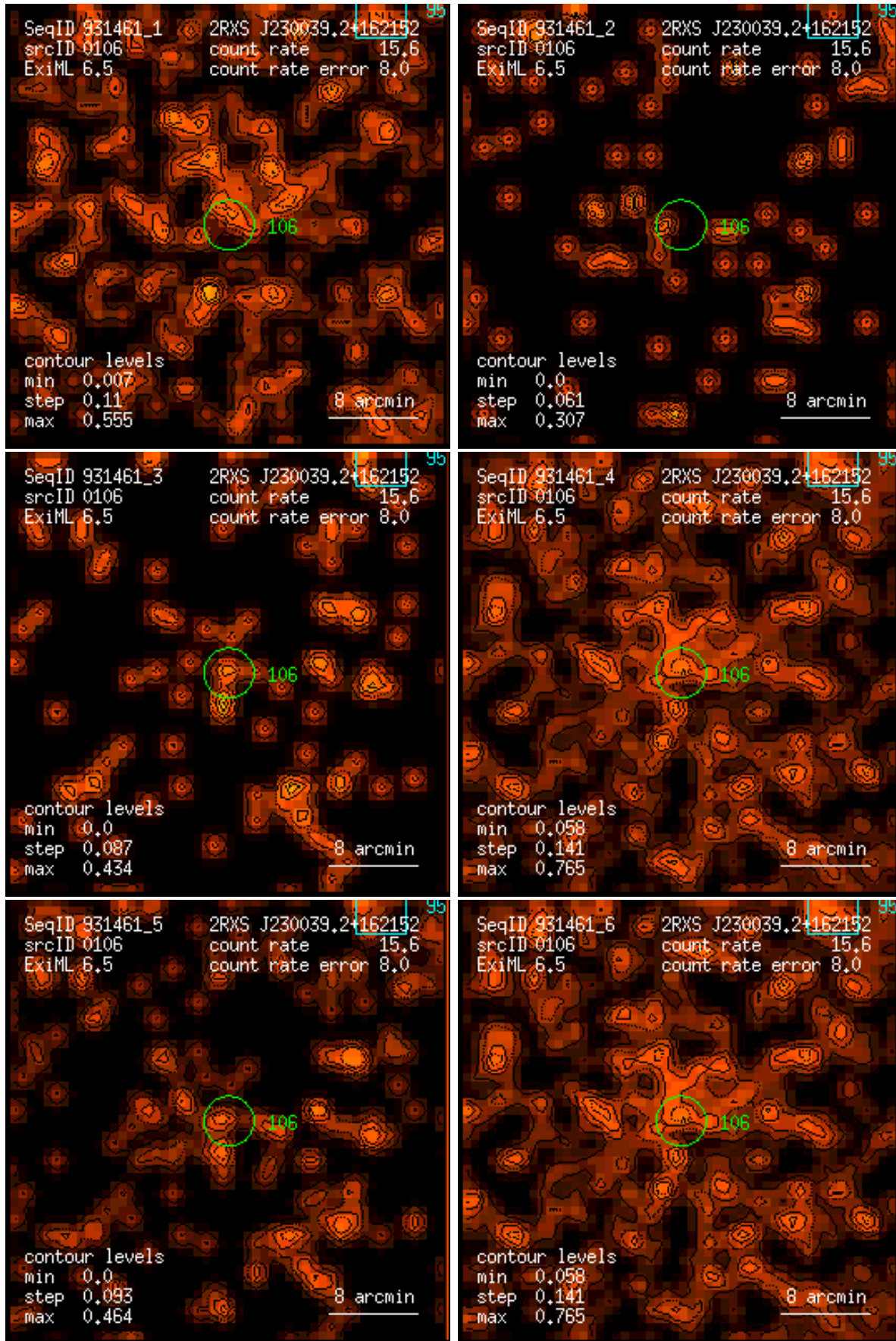
Figure 106: RASS 931461: detection 0106: band rate images, Gaussian filter: (1) PSPC channels 11 – 41, (2) 52 – 90, (3) 91 – 201, (4) 11 – 235, (5) 52 – 201, (6) 11 – 201. Broad band rates in counts/ks. Band rate contour levels in counts/ks/arcmin 2 .
