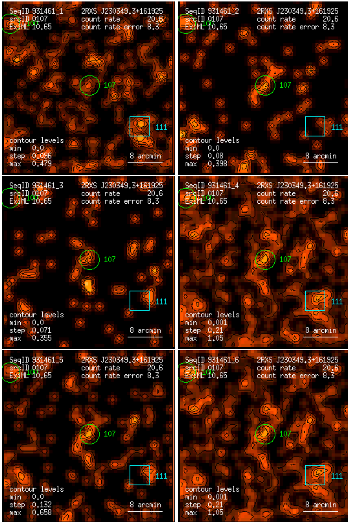
Figure 107: RASS 931461: detection 0107: band rate images, Gaussian filter: (1) PSPC channels 11 – 41, (2) 52 – 90, (3) 91 – 201, (4) 11 – 235, (5) 52 – 201, (6) 11 – 201. Broad band rates in counts/ks. Band rate contour levels in counts/ks/arcmin 2 .
