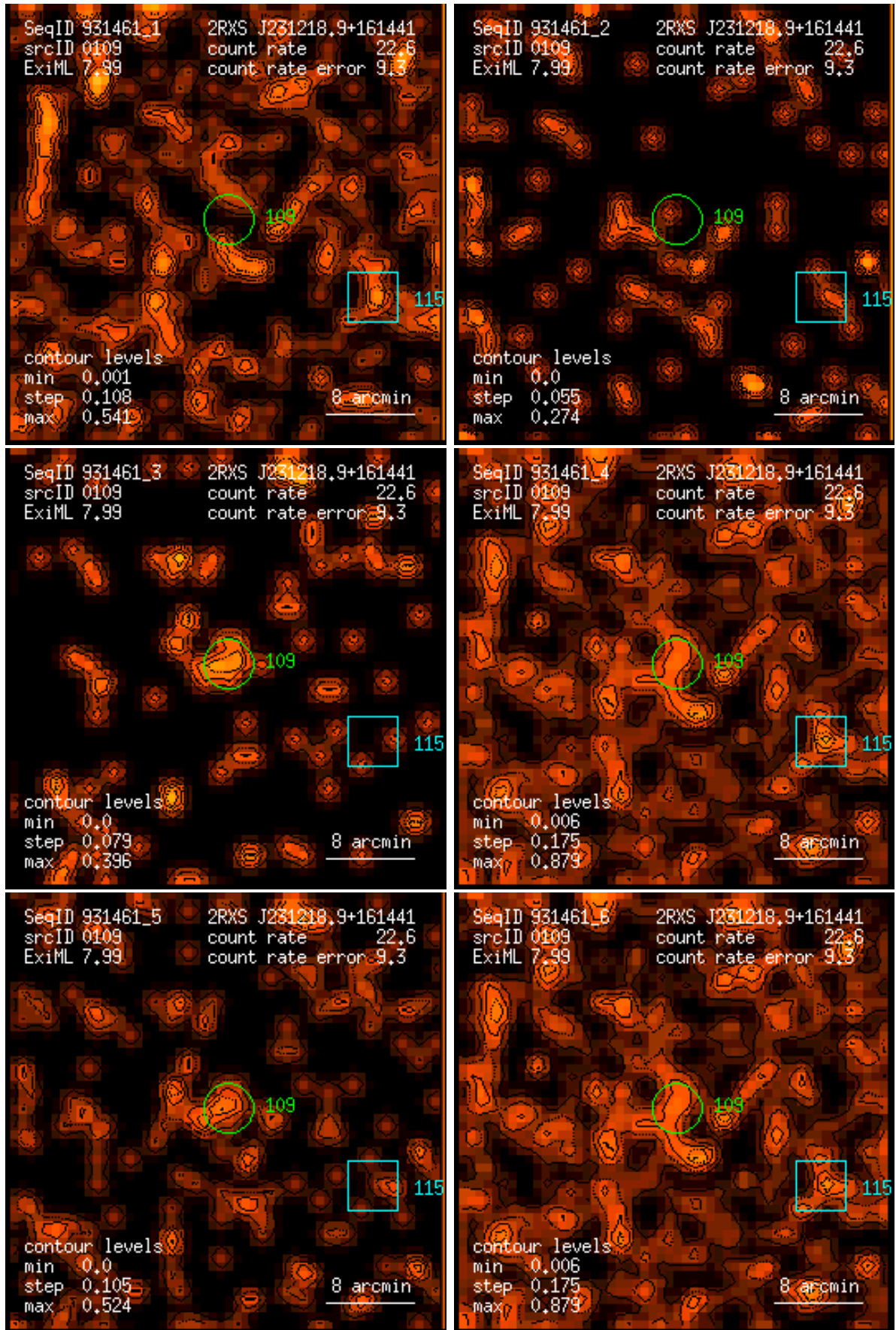
Figure 109: RASS 931461: detection 0109: band rate images, Gaussian filter: (1) PSPC channels 11 – 41, (2) 52 – 90, (3) 91 – 201, (4) 11 – 235, (5) 52 – 201, (6) 11 – 201. Broad band rates in counts/ks. Band rate contour levels in counts/ks/arcmin 2 .
