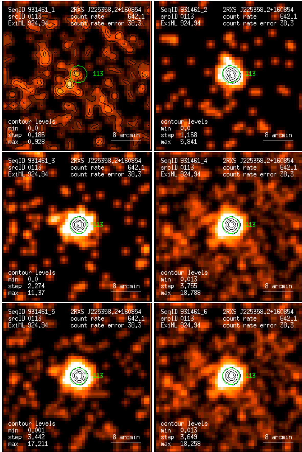
Figure 113: RASS 931461: detection 0113: band rate images, Gaussian filter: (1) PSPC channels 11 – 41, (2) 52 – 90, (3) 91 – 201, (4) 11 – 235, (5) 52 – 201, (6) 11 – 201. Broad band rates in counts/ks. Band rate contour levels in counts/ks/arcmin 2 .
