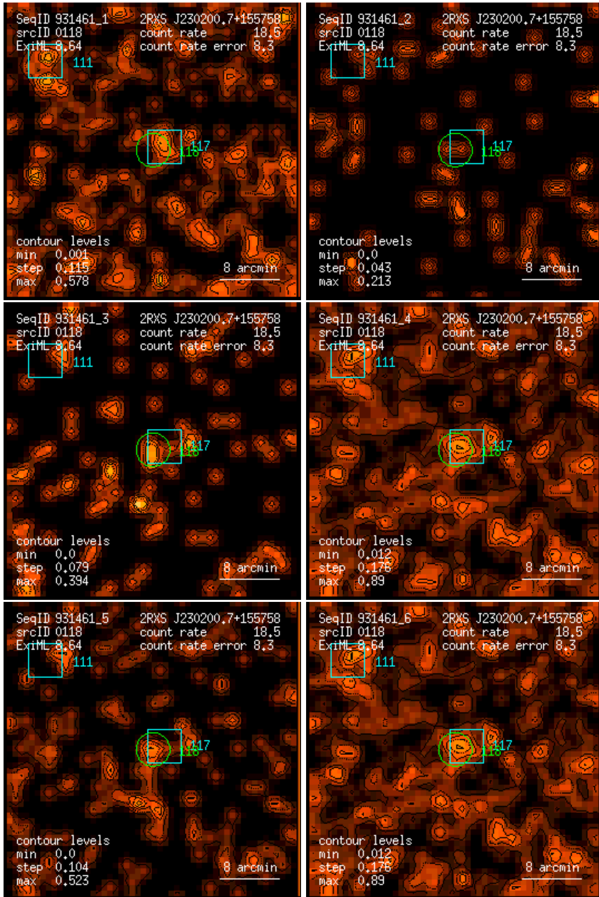
Figure 118: RASS 931461: detection 0118: band rate images, Gaussian filter: (1) PSPC channels 11 – 41, (2) 52 – 90, (3) 91 – 201, (4) 11 – 235, (5) 52 – 201, (6) 11 – 201. Broad band rates in counts/ks. Band rate contour levels in counts/ks/arcmin 2 .
