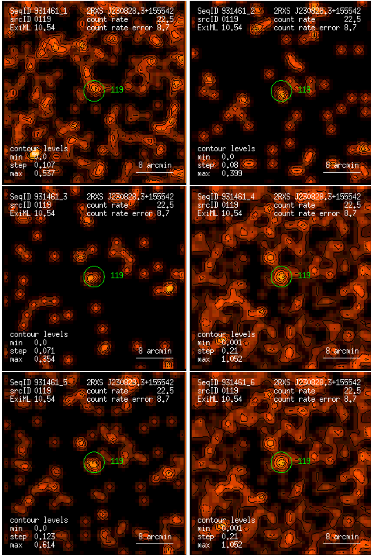
Figure 119: RASS 931461: detection 0119: band rate images, Gaussian filter: (1) PSPC channels 11 – 41, (2) 52 – 90, (3) 91 – 201, (4) 11 – 235, (5) 52 – 201, (6) 11 – 201. Broad band rates in counts/ks. Band rate contour levels in counts/ks/arcmin 2 .
