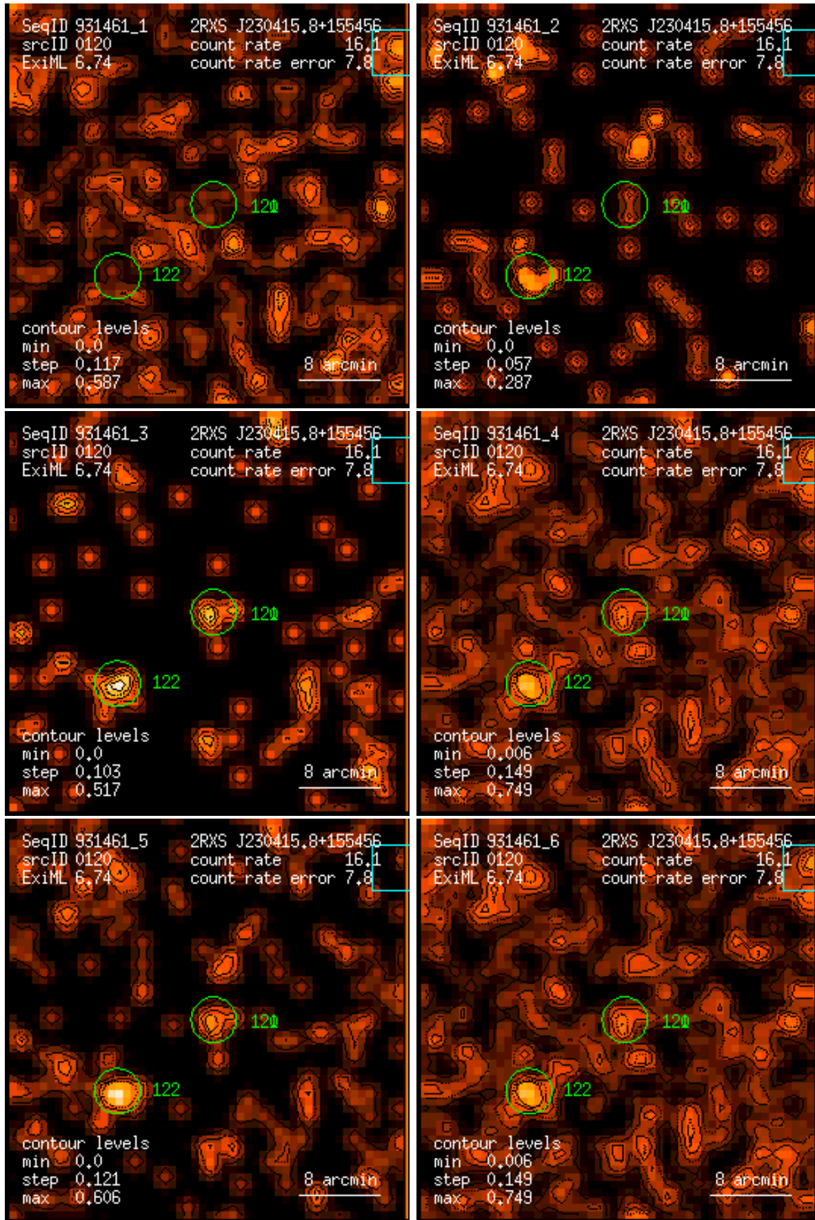
Figure 120: RASS 931461: detection 0120: band rate images, Gaussian filter: (1) PSPC channels 11 – 41, (2) 52 – 90, (3) 91 – 201, (4) 11 – 235, (5) 52 – 201, (6) 11 – 201. Broad band rates in counts/ks. Band rate contour levels in counts/ks/arcmin 2 .
