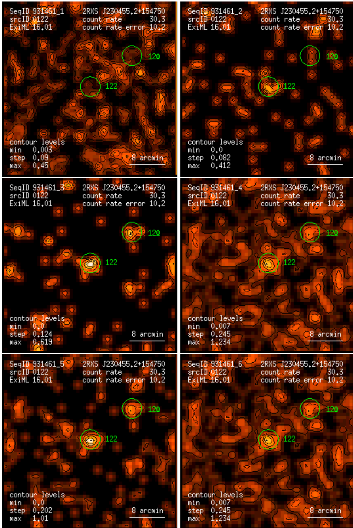
Figure 122: RASS 931461: detection 0122: band rate images, Gaussian filter: (1) PSPC channels 11 – 41, (2) 52 – 90, (3) 91 – 201, (4) 11 – 235, (5) 52 – 201, (6) 11 – 201. Broad band rates in counts/ks. Band rate contour levels in counts/ks/arcmin 2 .
