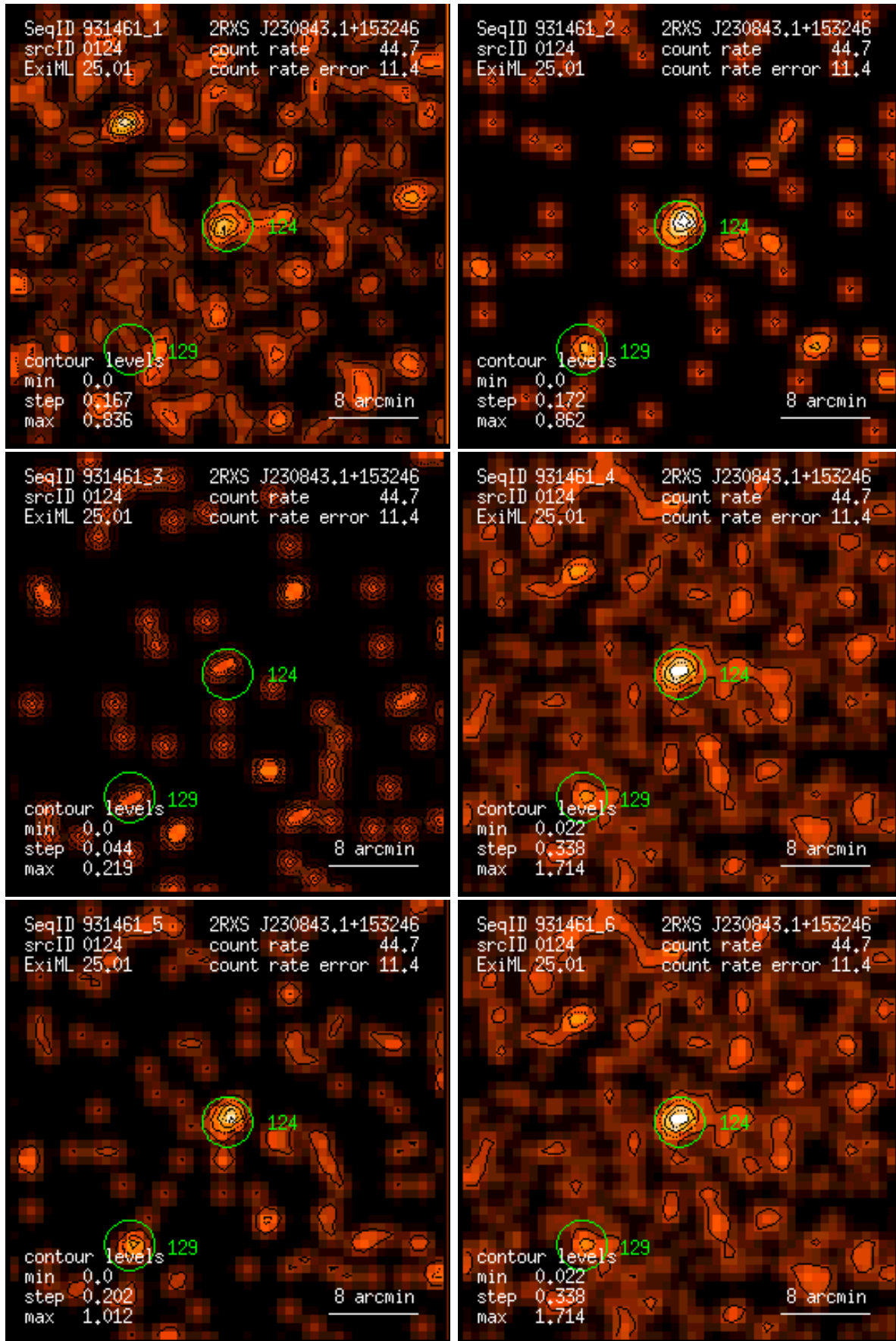
Figure 124: RASS 931461: detection 0124: band rate images, Gaussian filter: (1) PSPC channels 11 – 41, (2) 52 – 90, (3) 91 – 201, (4) 11 – 235, (5) 52 – 201, (6) 11 – 201. Broad band rates in counts/ks. Band rate contour levels in counts/ks/arcmin 2 .
