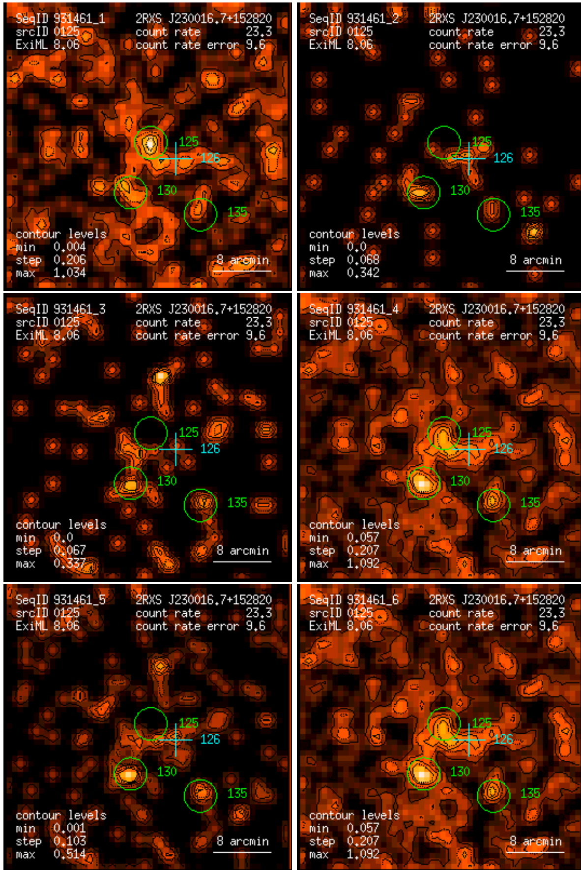
Figure 125: RASS 931461: detection 0125: band rate images, Gaussian filter: (1) PSPC channels 11 – 41, (2) 52 – 90, (3) 91 – 201, (4) 11 – 235, (5) 52 – 201, (6) 11 – 201. Broad band rates in counts/ks. Band rate contour levels in counts/ks/arcmin 2 .
