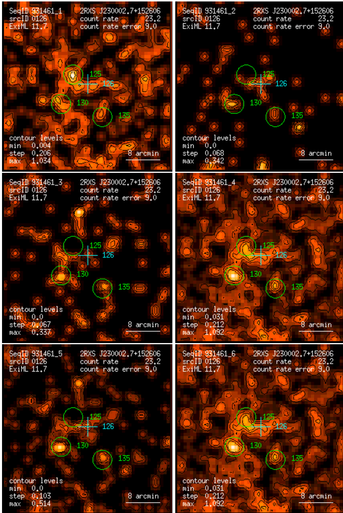
Figure 126: RASS 931461: detection 0126: band rate images, Gaussian filter: (1) PSPC channels 11 – 41, (2) 52 – 90, (3) 91 – 201, (4) 11 – 235, (5) 52 – 201, (6) 11 – 201. Broad band rates in counts/ks. Band rate contour levels in counts/ks/arcmin 2 .
