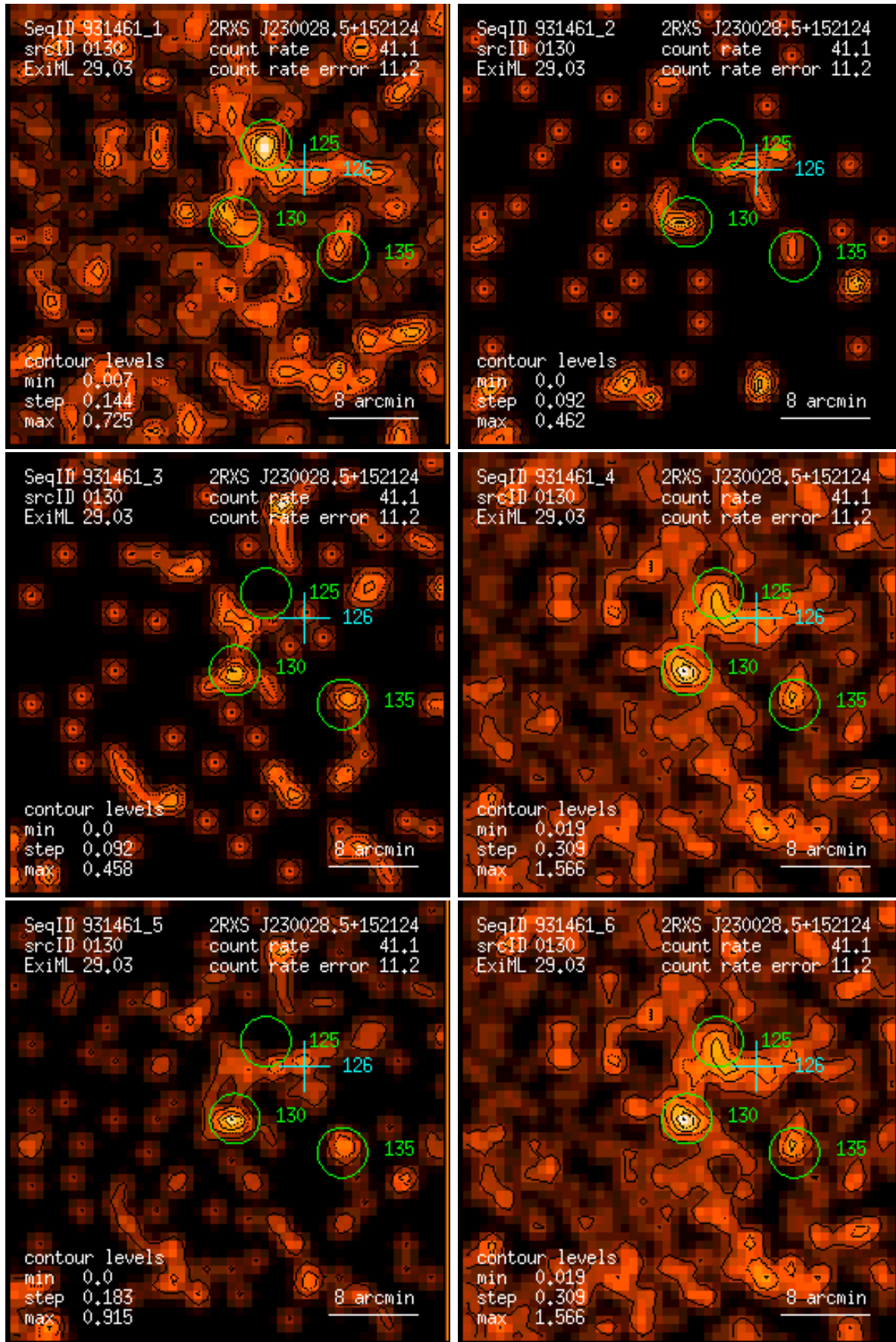
Figure 130: RASS 931461: detection 0130: band rate images, Gaussian filter: (1) PSPC channels 11 – 41, (2) 52 – 90, (3) 91 – 201, (4) 11 – 235, (5) 52 – 201, (6) 11 – 201. Broad band rates in counts/ks. Band rate contour levels in counts/ks/arcmin 2 .
