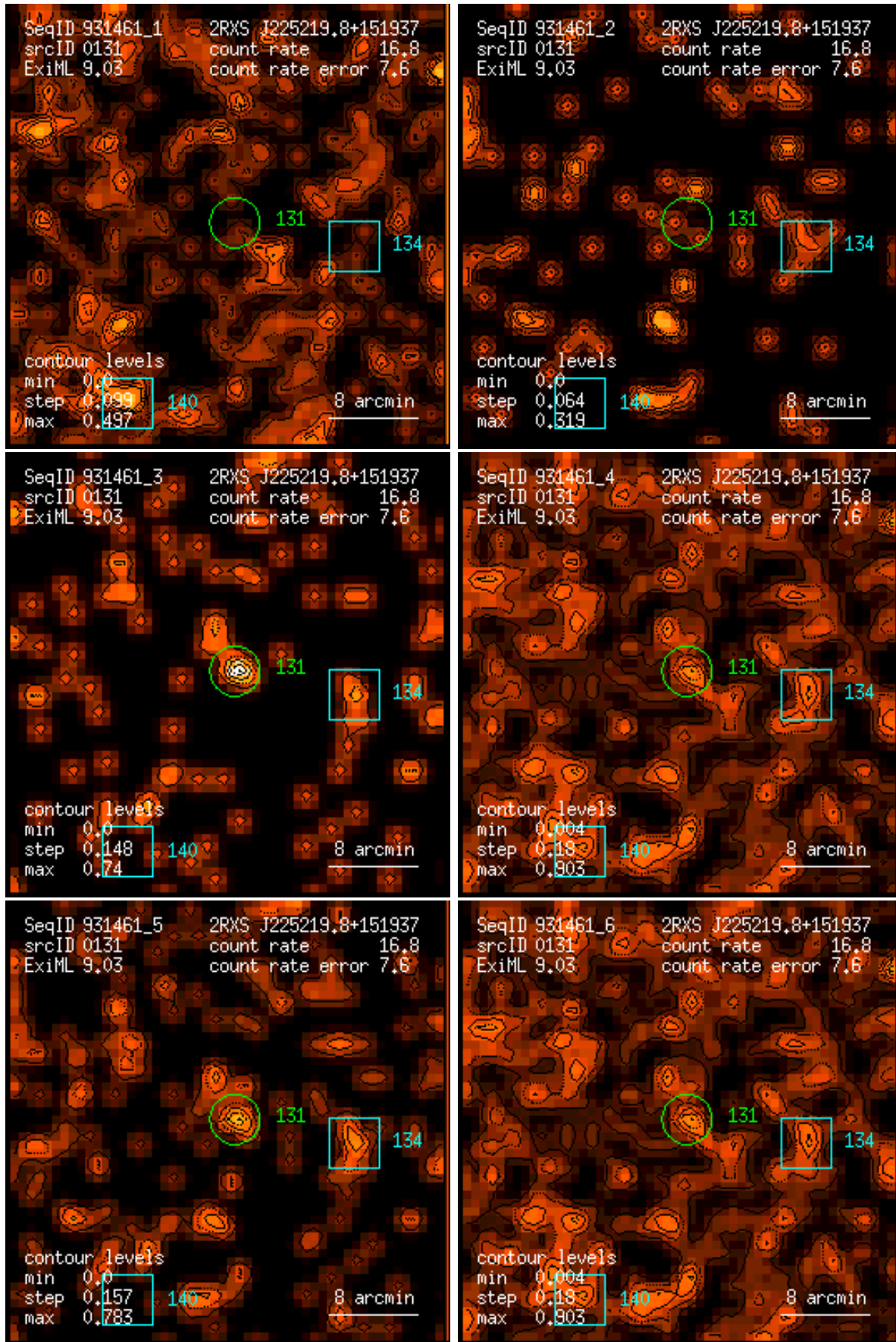
Figure 131: RASS 931461: detection 0131: band rate images, Gaussian filter: (1) PSPC channels 11 – 41, (2) 52 – 90, (3) 91 – 201, (4) 11 – 235, (5) 52 – 201, (6) 11 – 201. Broad band rates in counts/ks. Band rate contour levels in counts/ks/arcmin 2 .
