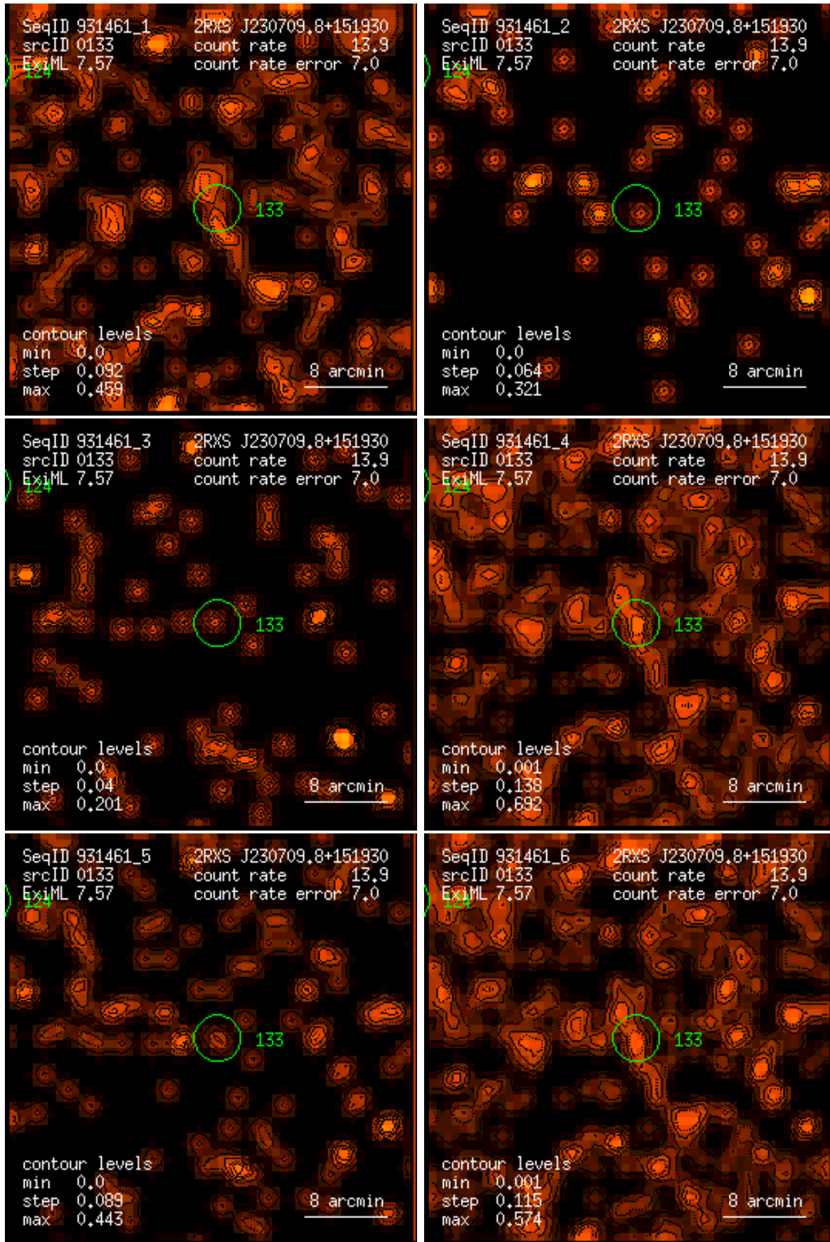
Figure 133: RASS 931461: detection 0133: band rate images, Gaussian filter: (1) PSPC channels 11 – 41, (2) 52 – 90, (3) 91 – 201, (4) 11 – 235, (5) 52 – 201, (6) 11 – 201. Broad band rates in counts/ks. Band rate contour levels in counts/ks/arcmin 2 .
