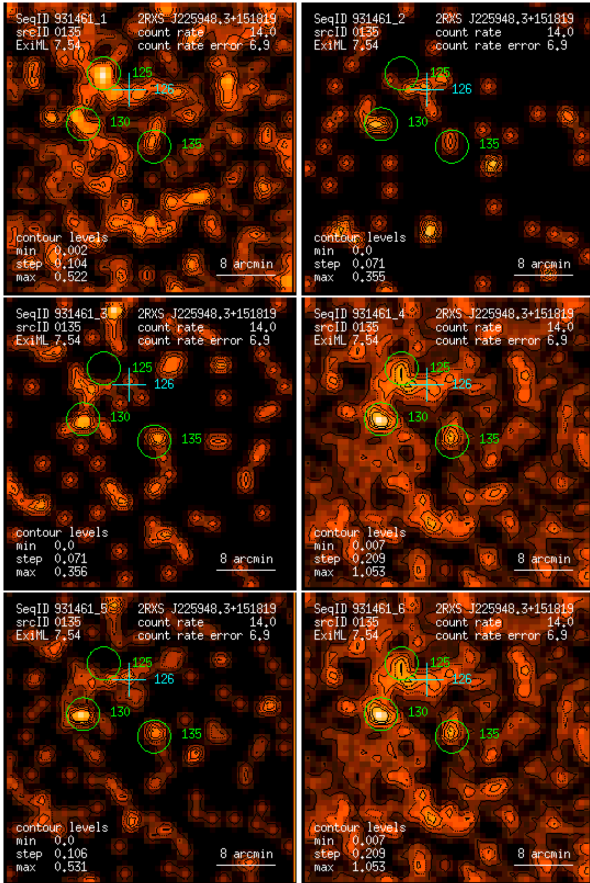
Figure 135: RASS 931461: detection 0135: band rate images, Gaussian filter: (1) PSPC channels 11 – 41, (2) 52 – 90, (3) 91 – 201, (4) 11 – 235, (5) 52 – 201, (6) 11 – 201. Broad band rates in counts/ks. Band rate contour levels in counts/ks/arcmin 2 .
