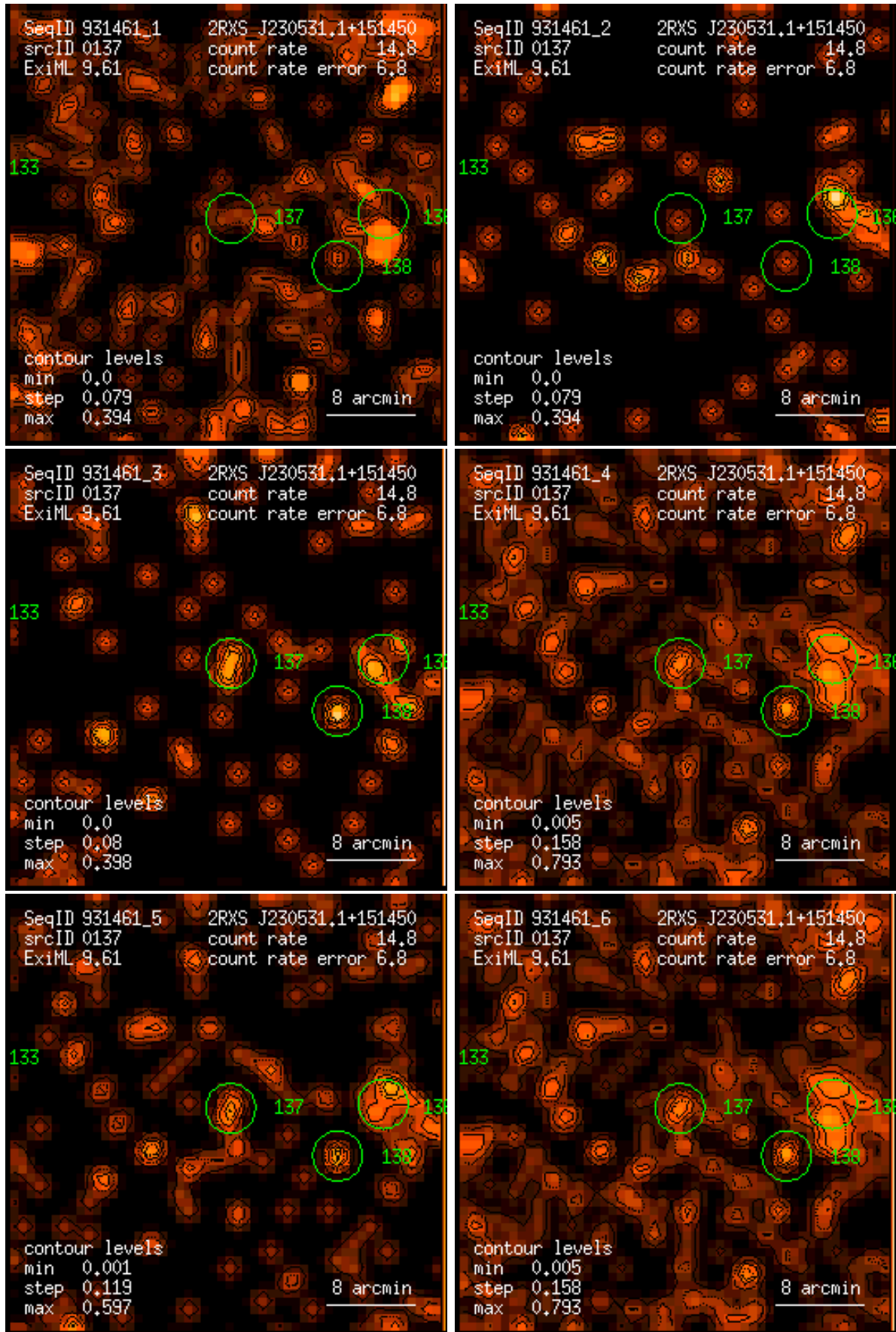
Figure 137: RASS 931461: detection 0137: band rate images, Gaussian filter: (1) PSPC channels 11 – 41, (2) 52 – 90, (3) 91 – 201, (4) 11 – 235, (5) 52 – 201, (6) 11 – 201. Broad band rates in counts/ks. Band rate contour levels in counts/ks/arcmin 2 .
