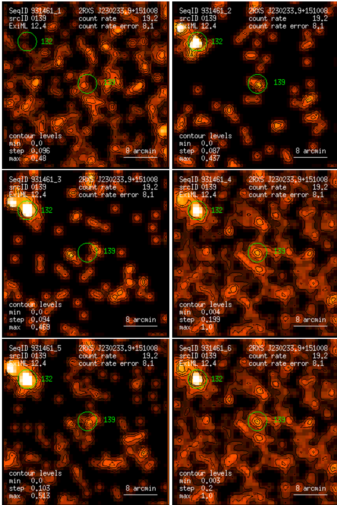
Figure 139: RASS 931461: detection 0139: band rate images, Gaussian filter: (1) PSPC channels 11 – 41, (2) 52 – 90, (3) 91 – 201, (4) 11 – 235, (5) 52 – 201, (6) 11 – 201. Broad band rates in counts/ks. Band rate contour levels in counts/ks/arcmin 2 .
