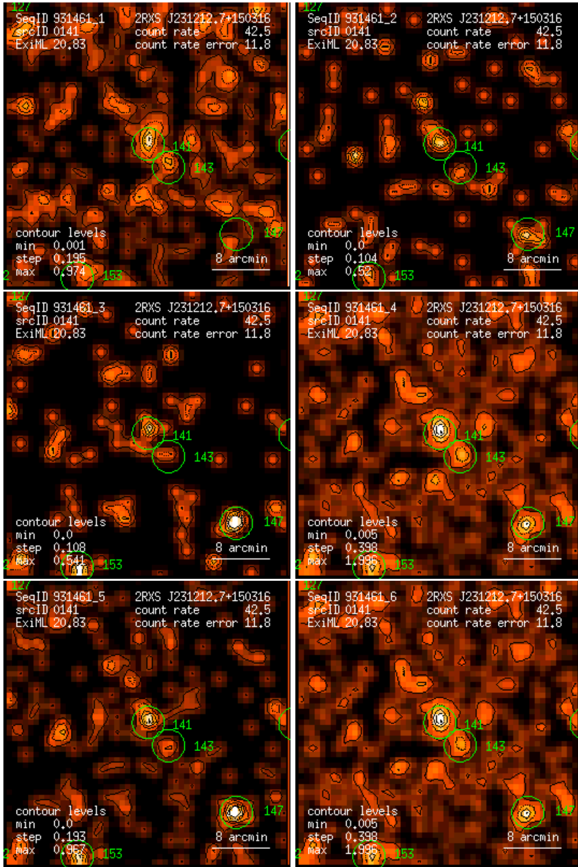
Figure 141: RASS 931461: detection 0141: band rate images, Gaussian filter: (1) PSPC channels 11 – 41, (2) 52 – 90, (3) 91 – 201, (4) 11 – 235, (5) 52 – 201, (6) 11 – 201. Broad band rates in counts/ks. Band rate contour levels in counts/ks/arcmin 2 .
