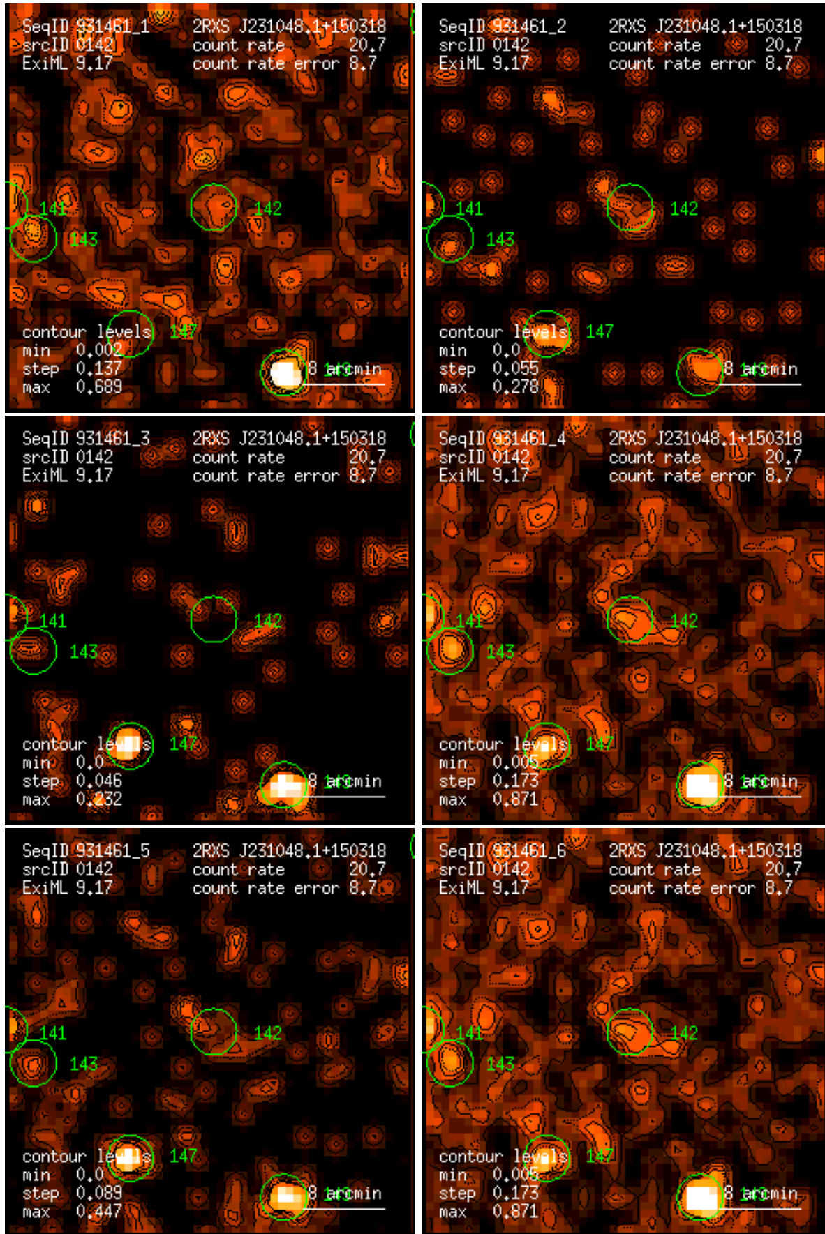
Figure 142: RASS 931461: detection 0142: band rate images, Gaussian filter: (1) PSPC channels 11 – 41, (2) 52 – 90, (3) 91 – 201, (4) 11 – 235, (5) 52 – 201, (6) 11 – 201. Broad band rates in counts/ks. Band rate contour levels in counts/ks/arcmin 2 .
