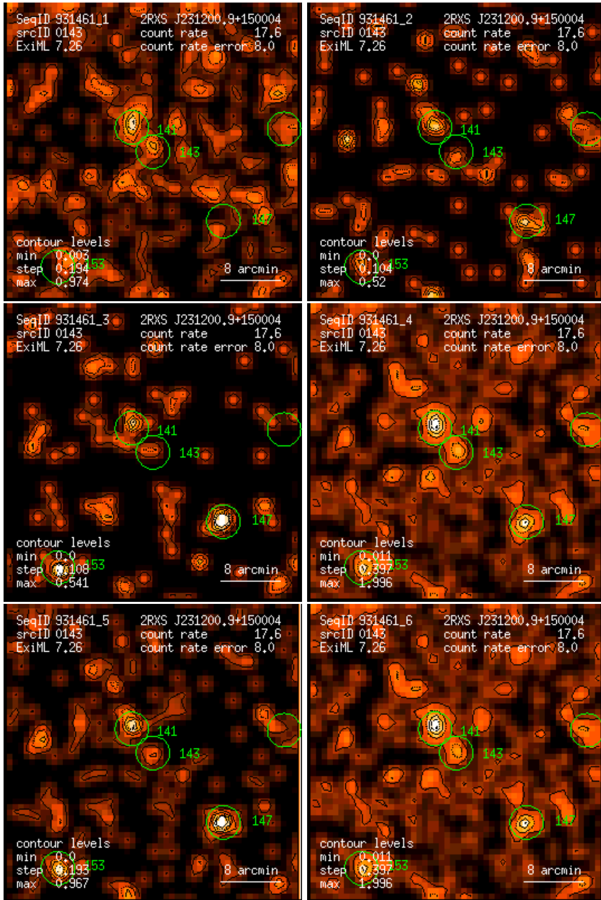
Figure 143: RASS 931461: detection 0143: band rate images, Gaussian filter: (1) PSPC channels 11 – 41, (2) 52 – 90, (3) 91 – 201, (4) 11 – 235, (5) 52 – 201, (6) 11 – 201. Broad band rates in counts/ks. Band rate contour levels in counts/ks/arcmin 2 .
