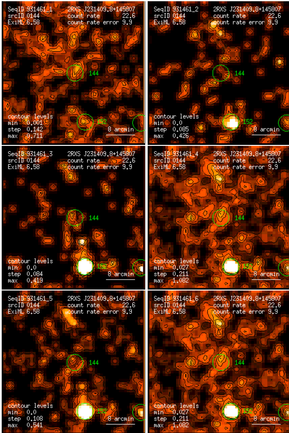
Figure 144: RASS 931461: detection 0144: band rate images, Gaussian filter: (1) PSPC channels 11 – 41, (2) 52 – 90, (3) 91 – 201, (4) 11 – 235, (5) 52 – 201, (6) 11 – 201. Broad band rates in counts/ks. Band rate contour levels in counts/ks/arcmin 2 .
