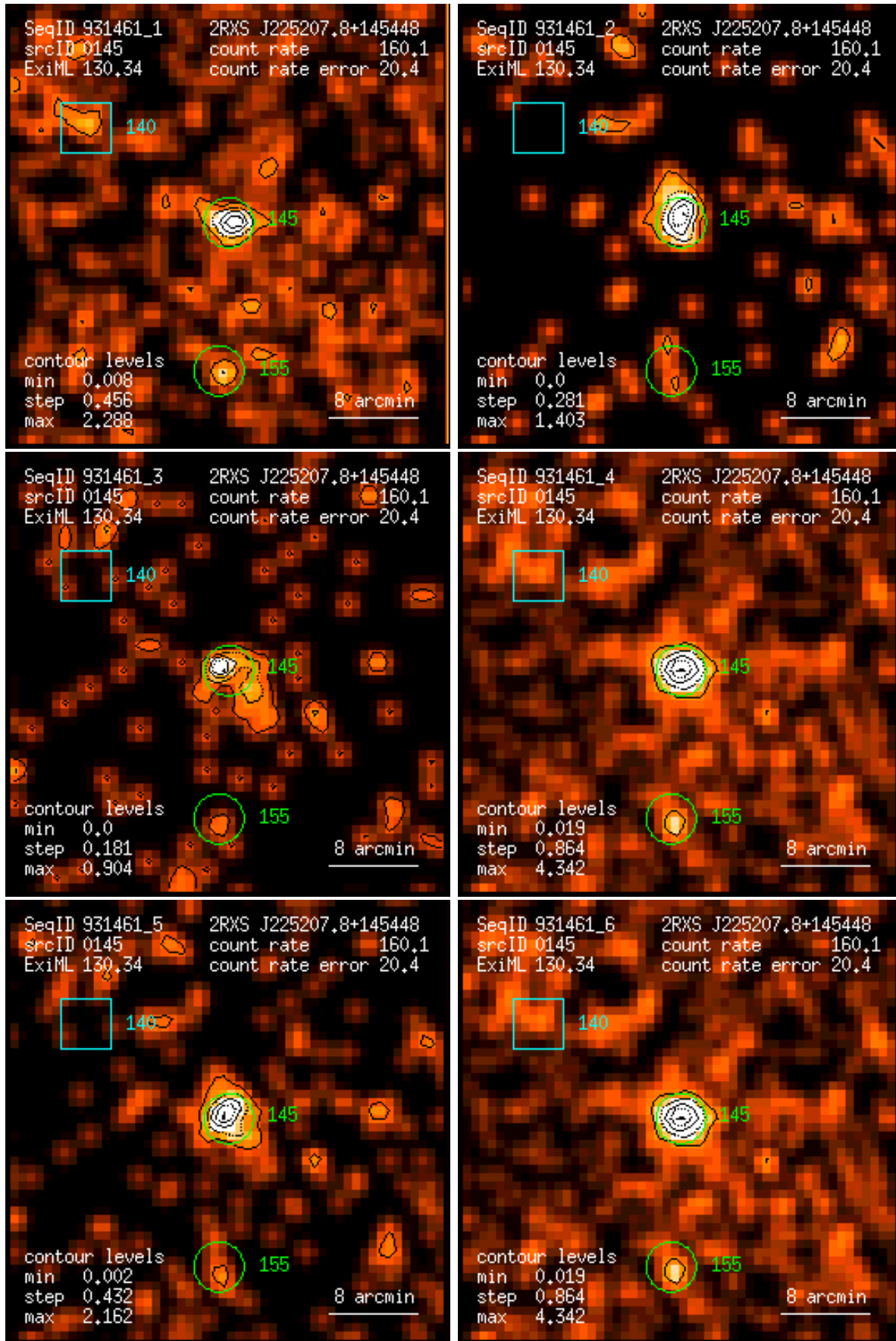
Figure 145: RASS 931461: detection 0145: band rate images, Gaussian filter: (1) PSPC channels 11 – 41, (2) 52 – 90, (3) 91 – 201, (4) 11 – 235, (5) 52 – 201, (6) 11 – 201. Broad band rates in counts/ks. Band rate contour levels in counts/ks/arcmin 2 .
